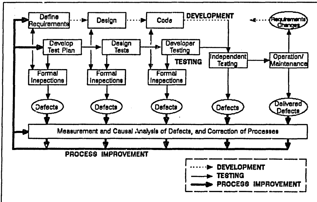
Figure 1. Software Quality Control
