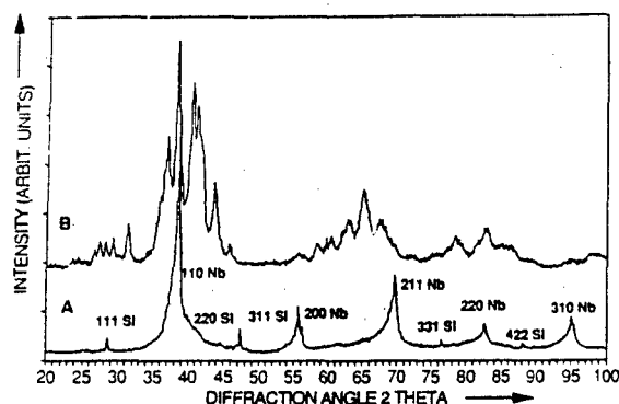
Fig. 3. X-ray diffraction patterns of mechanically alloyed Nb-Si powders: curve A, just before (3 h) compound formation; curve B, just after (3 h 15 min) compound formation.
