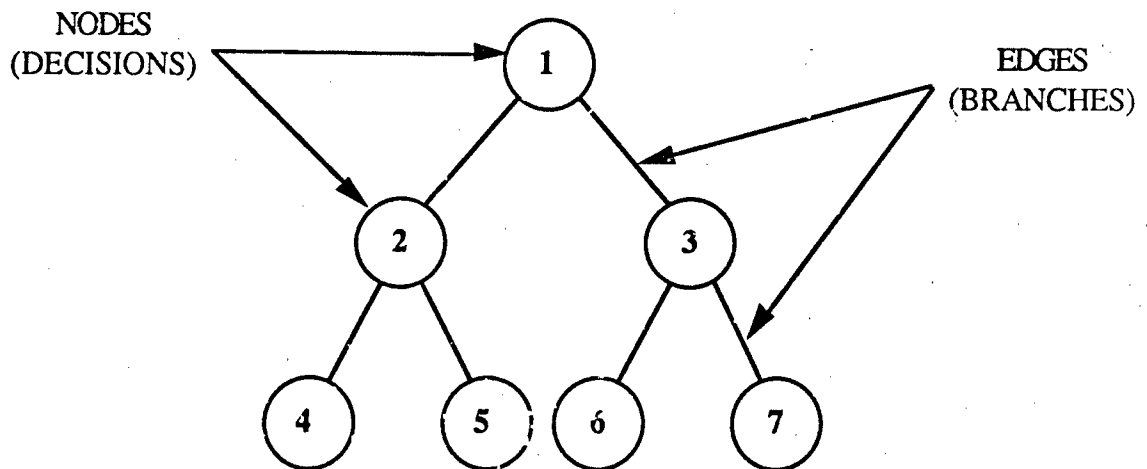
DIRECTED FLOW GRAPH FIGURE 1
