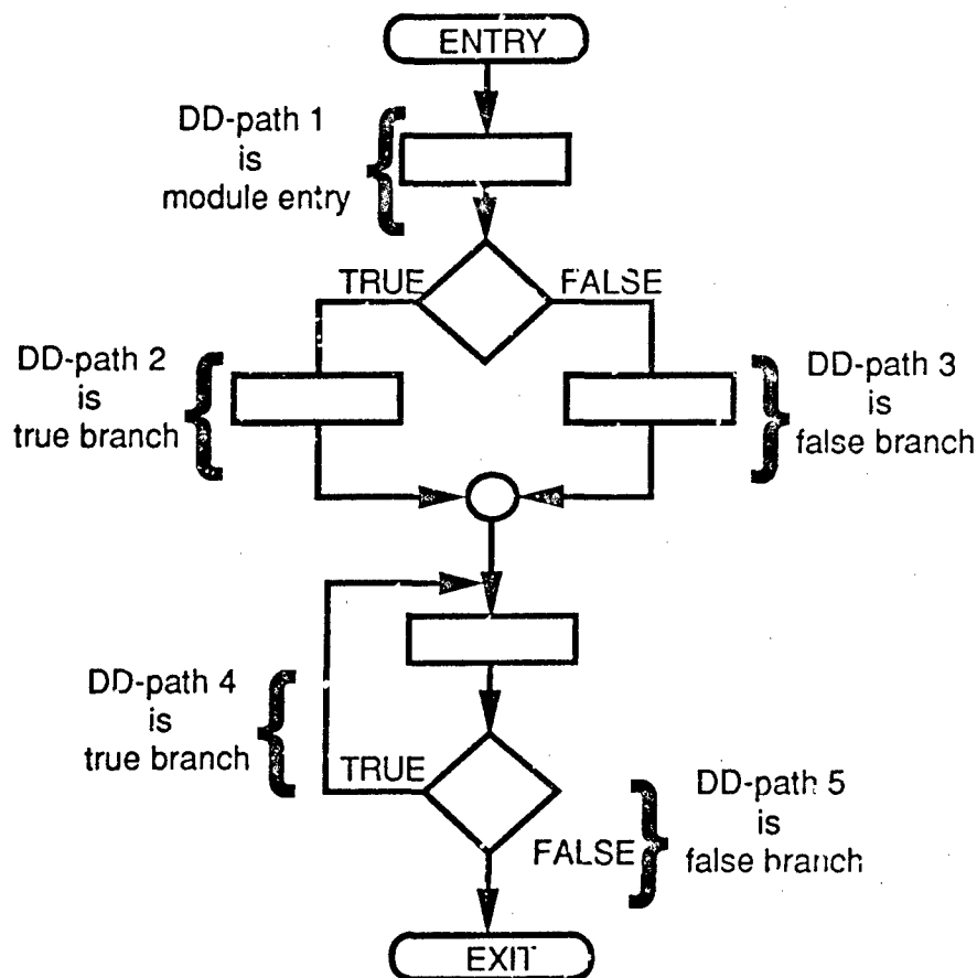
DECISION-TO-DECISION PATH EXAMPLE
