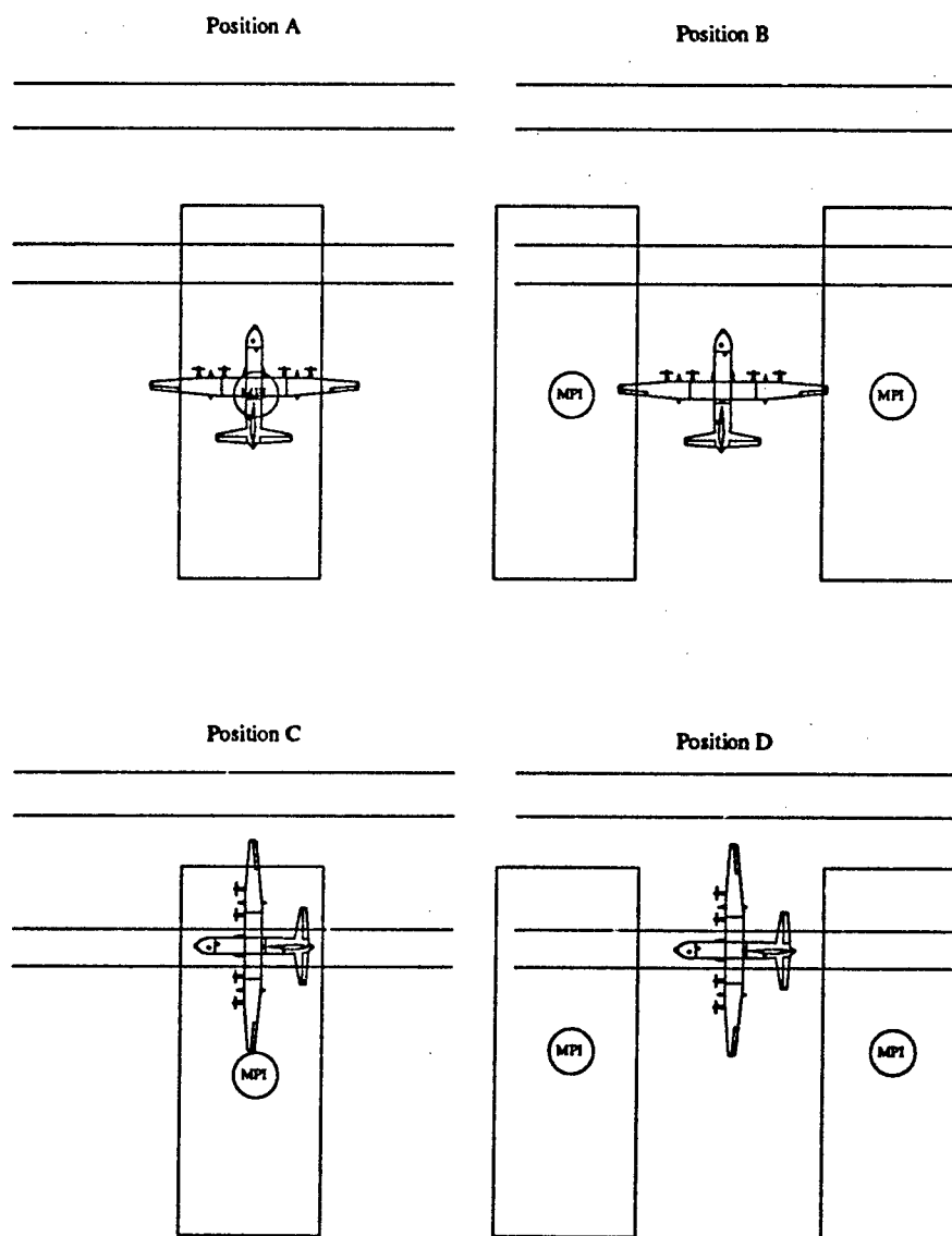
Figure 3.3. Aircraft position on airfield (Attack I).
