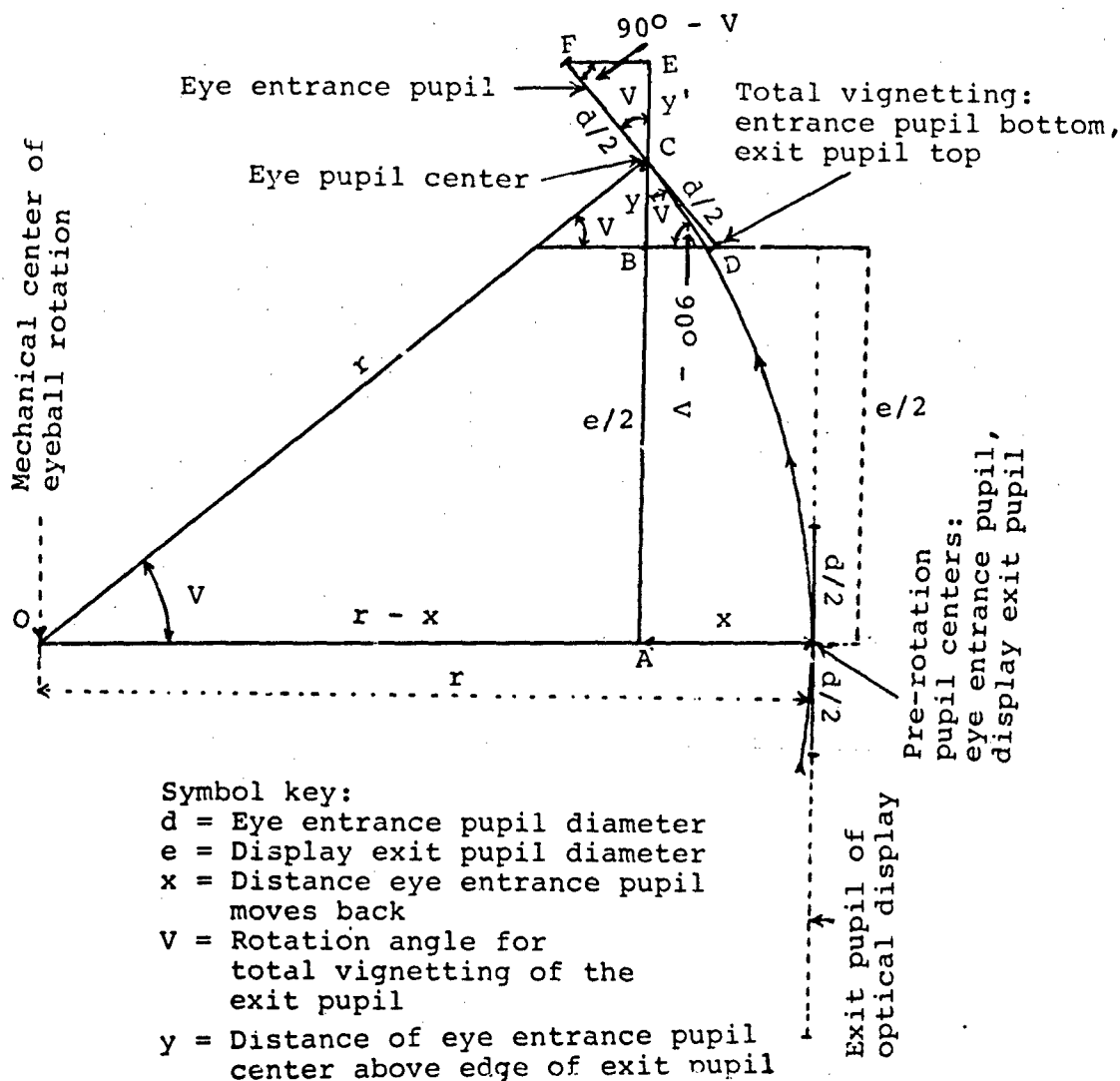
Fig. 5. Total vignetting of the display exit pupil. The figure is for a display exit pupil of 10mm and an eye entrance pupil of 3mm, providing complete vignetting at a rotation angle of 38.2 deg.
