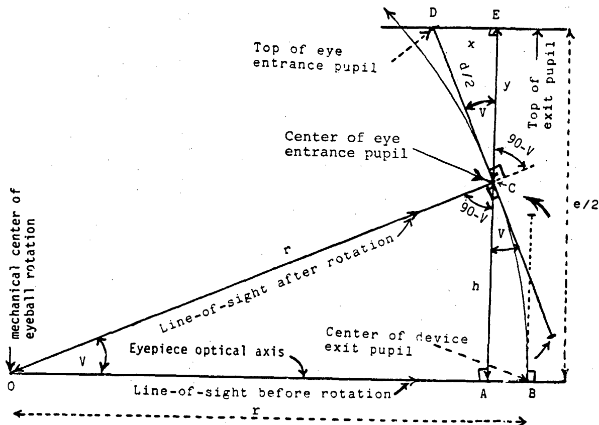
Fig. 6. Optical geometry at the start of exit pupil vignetting.
