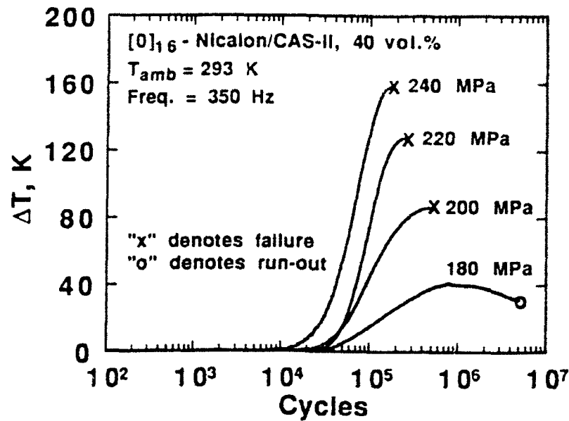
Fig. 5. Influence of maximum fatigue stress on the temperature rise ( T - T_{ambient} ) of [0] 16 -Nicalon/CAS-II composites fatigued at a sinusoidal loading frequency of 350 Hz.
