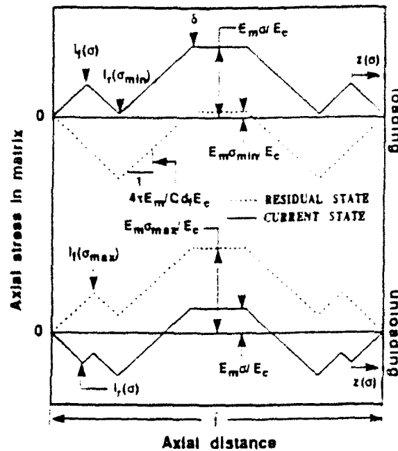
Fig. 3. Stress distribution in the matrix during loading and unloading for the case of partial slip. Loading is assumed to occur from \sigma_{min} to an intermediate stress \sigma . Unloading occurs from \sigma_{max} to \sigma .
