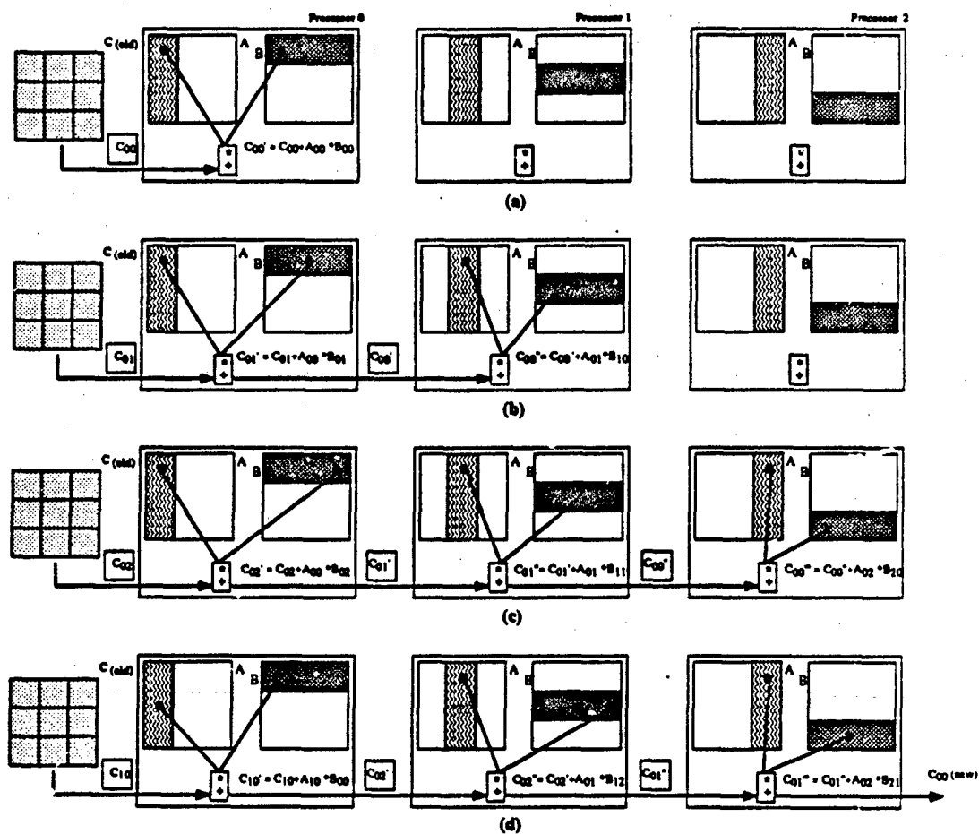
Figure 8: Parallel matrix multiplication based on systolic communication
