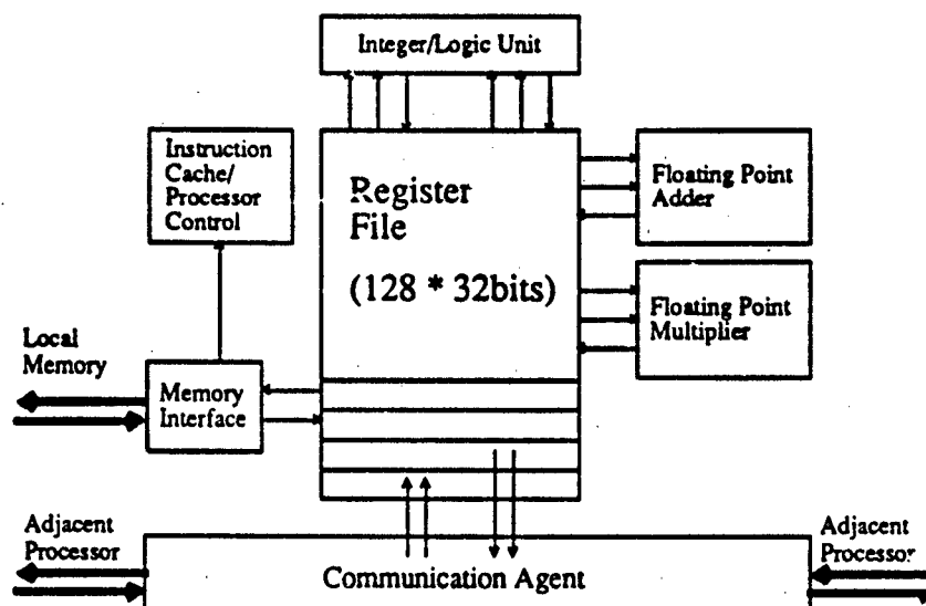
Figure 1: iWarp processor
