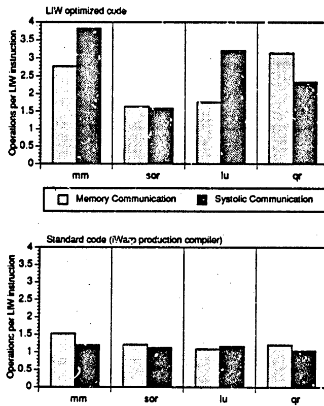
Figure 3: Operations per instruction, optimized (top) and standard (bottom).
