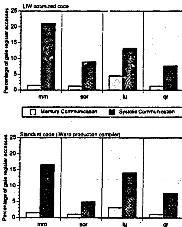
Figure 5: Percentage of register accesses through the gates
