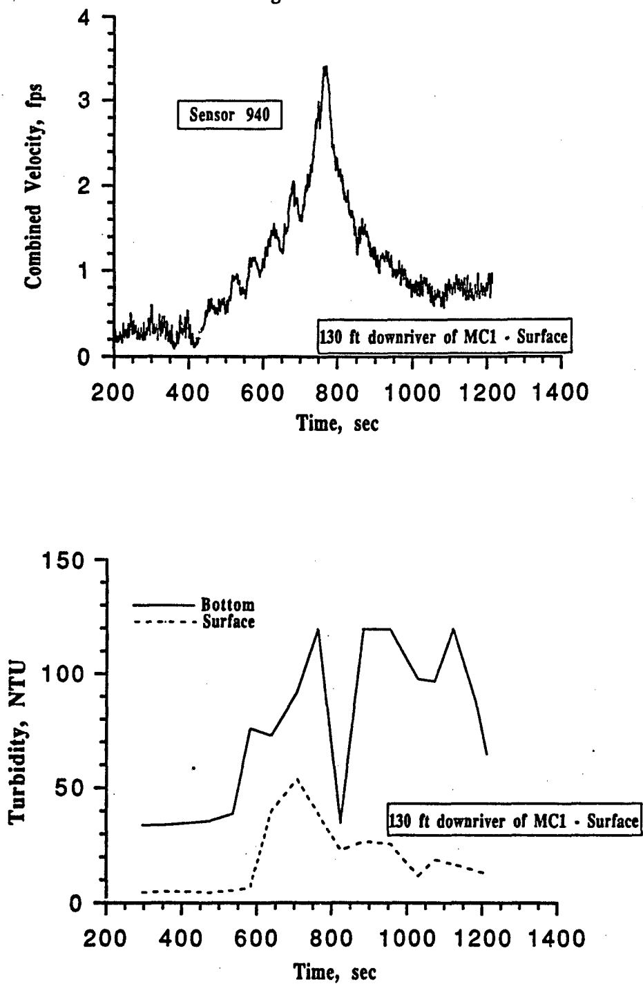
Figure 4. Combined velocity and changes in turbidity for Sensor 940, Test 6
