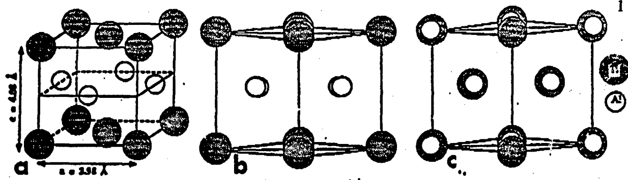
FIG. 1. (a) TlAl (L10) crystal structure with perspective views along (b) [110] and (c) [101] .
