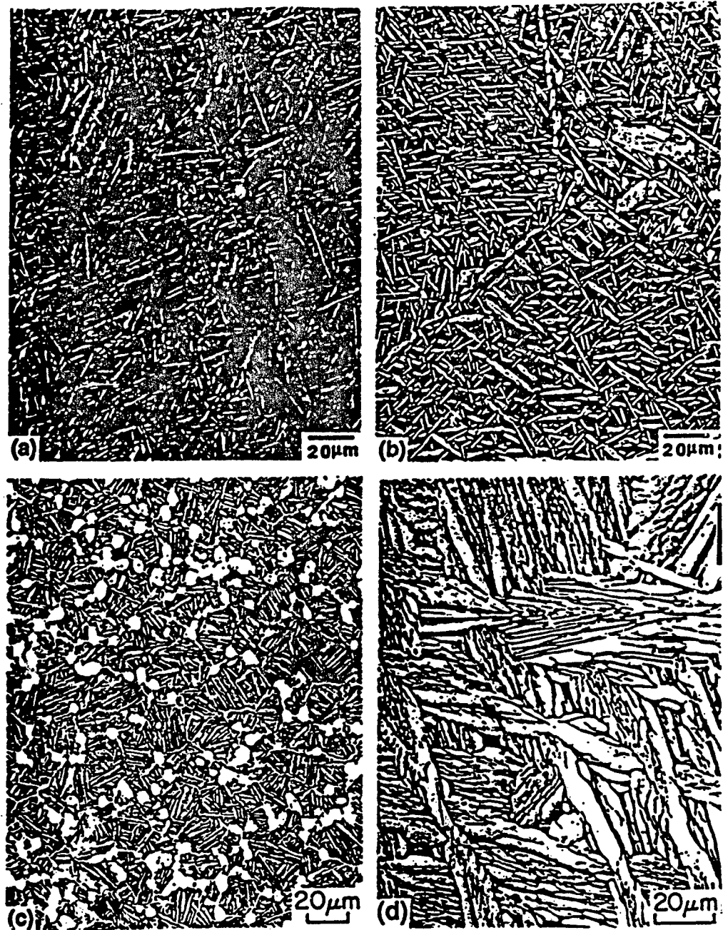
Fig. 1. Examples of microstructural range observed in \alpha_2 + \beta titanium aluminide alloys. (a) Widmanstätten or basketweave morphology of \alpha_2 plates, formed in Ti-25-10-3-1 on cooling from the \beta phase at 0.5 K/s. (b) Coarser Widmanstätten \alpha_2 plates, formed in Ti-25-10-3-1 on cooling from the \alpha_2 + \beta two-phase region at 0.5 K/s. (c) Primary \alpha_2 and "packet" \alpha_2 plates in Ti-25-10-3-1 cooled from the \alpha_2 + \beta two-phase region. (d) Colonies of \alpha_2 plates in Ti-24-11 cooled from 1000°C (low in the \alpha_2 + \beta two-phase region) at 5 K/s.
