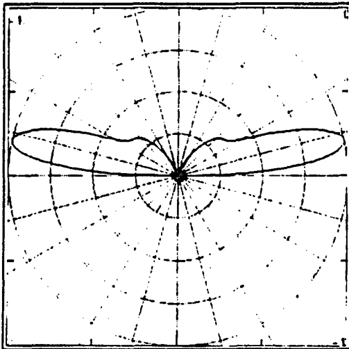
FIGURE 5.2: Vertical dipole space wave radiation pattern.
