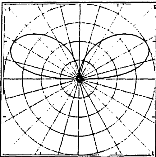
FIGURE 6.2: Monopole space wave radiation pattern.
