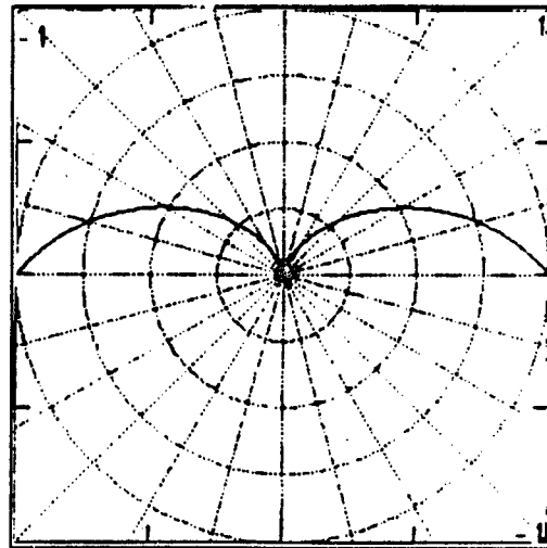
FIGURE 7.5: Horizontal dipole surface wave radiation pattern for \phi=\pi/2 vertical plane.
