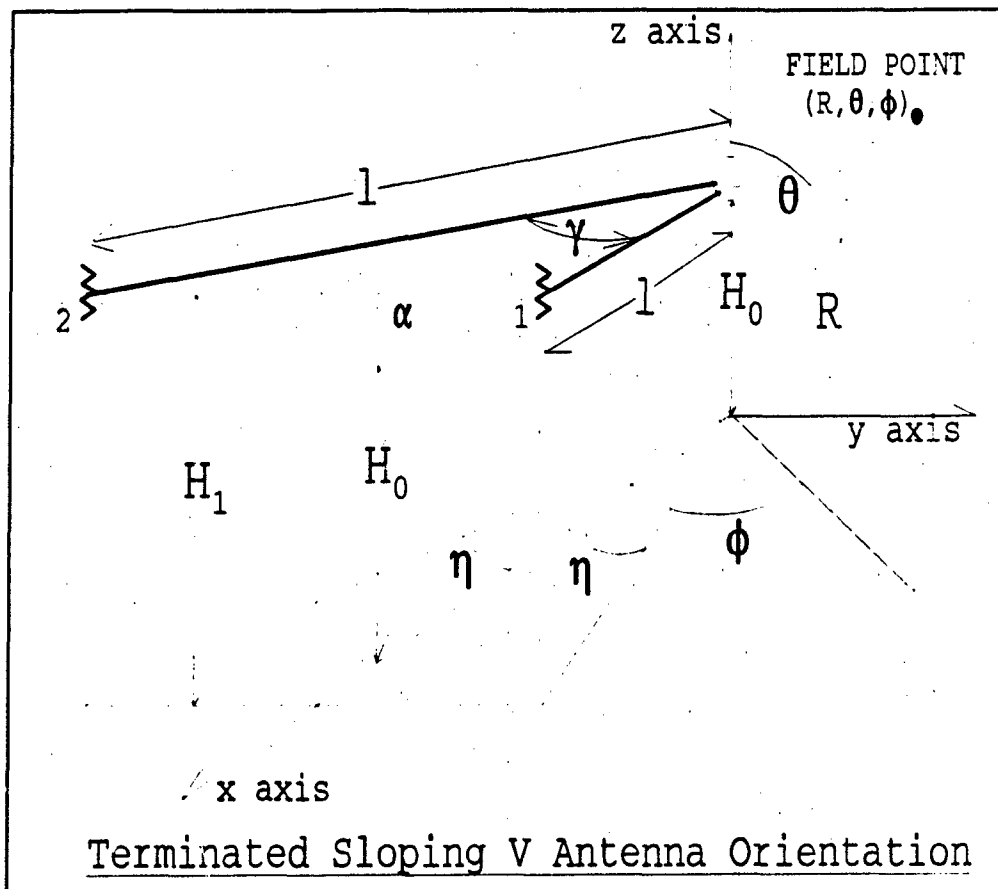
FIGURE 11.1: Spatial orientation of the terminated sloping V antenna for its corresponding Mathcad application.
