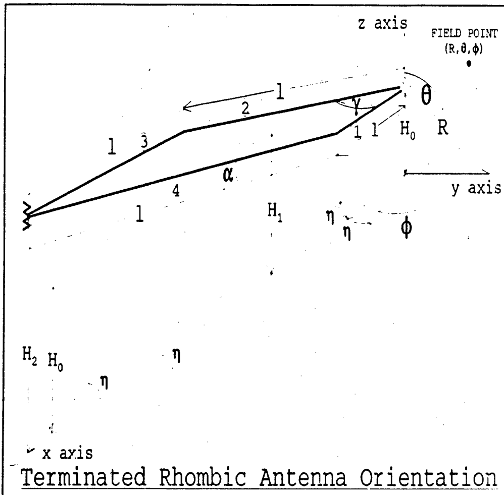
FIGURE 13.1: Spatial orientation of the terminated sloping or horizontal rhombic antenna for its Mathcad application.
