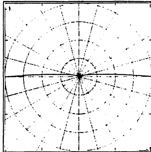
FIGURE 5.3: Vertical dipole surface wave pattern.
