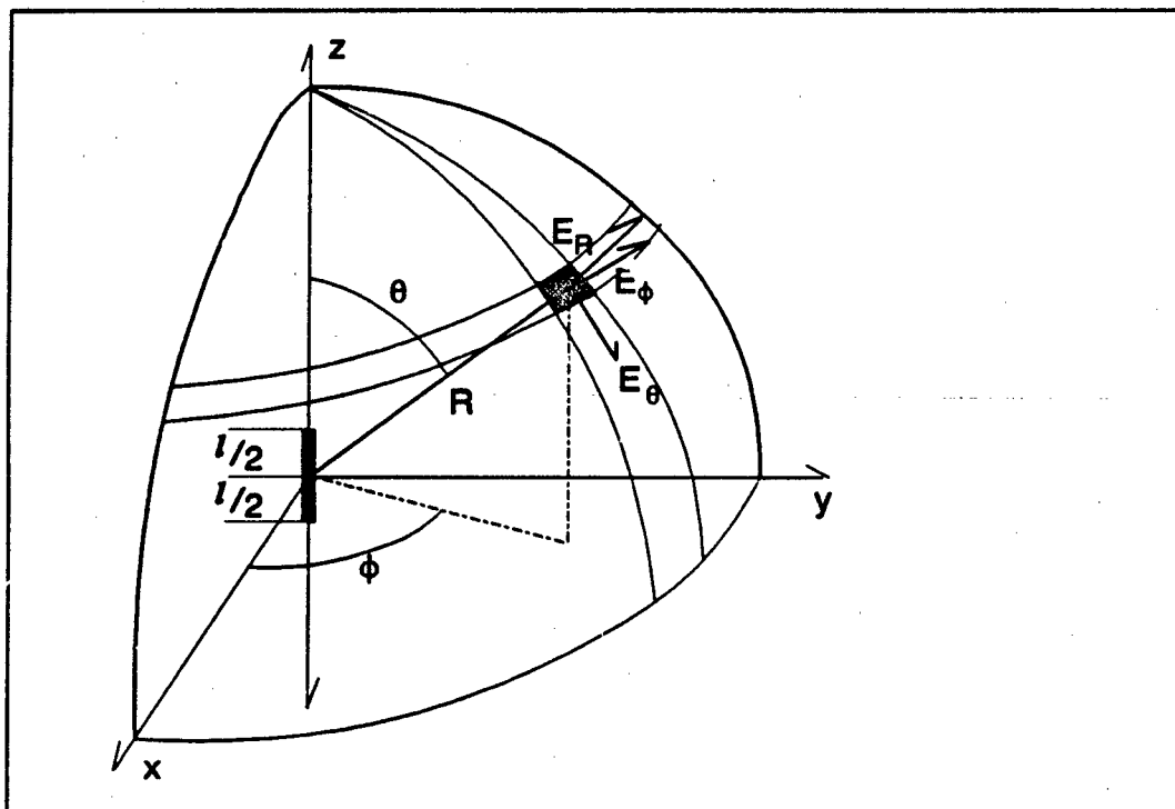
FIGURE 4.1: Elemental dipole spatial orientation.
