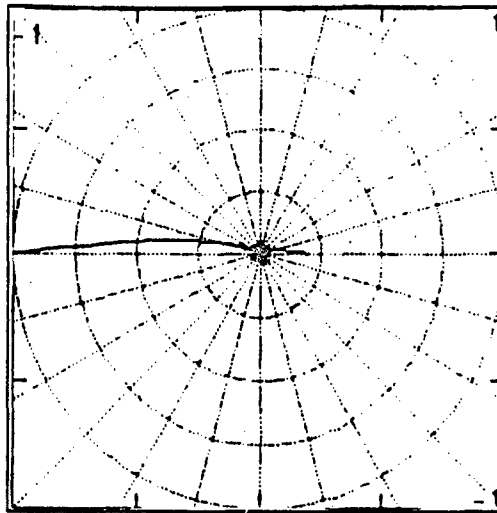
FIGURE 15.5: Vertical log-periodic surface wave radiation pattern for \phi=\pi/2 vertical plane.
