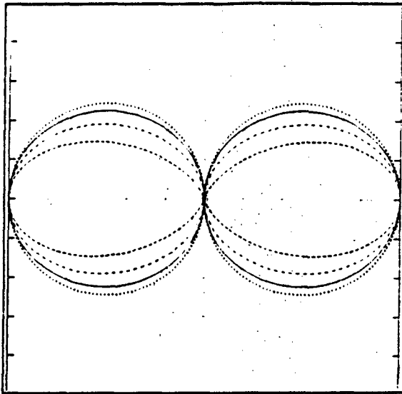
FIGURE 4.4: Vertical plane patterns for dipoles of length l = \lambda/4 ..... , l = \lambda/2 - · - · - , l = 3\lambda/4 - - - - , and l = \lambda - - - - .
