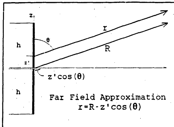
FIGURE 4.3: Phase approximation for distance variable, r .
