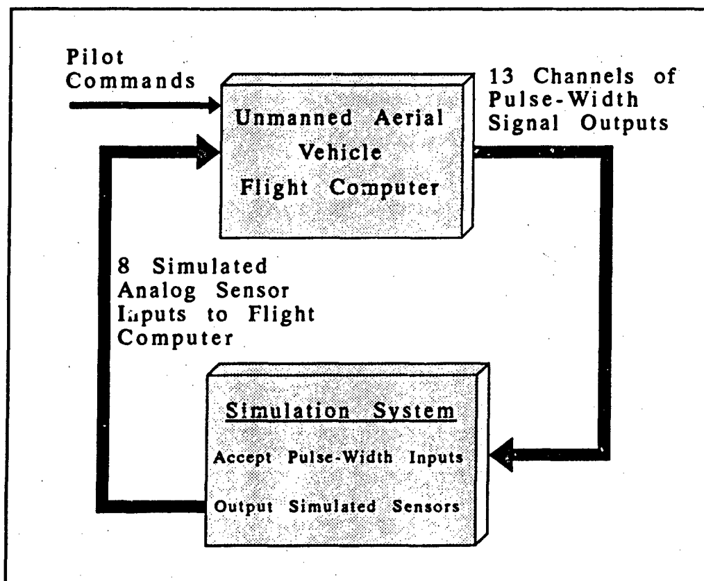
Figure 6: Top Level Simulation Architecture
