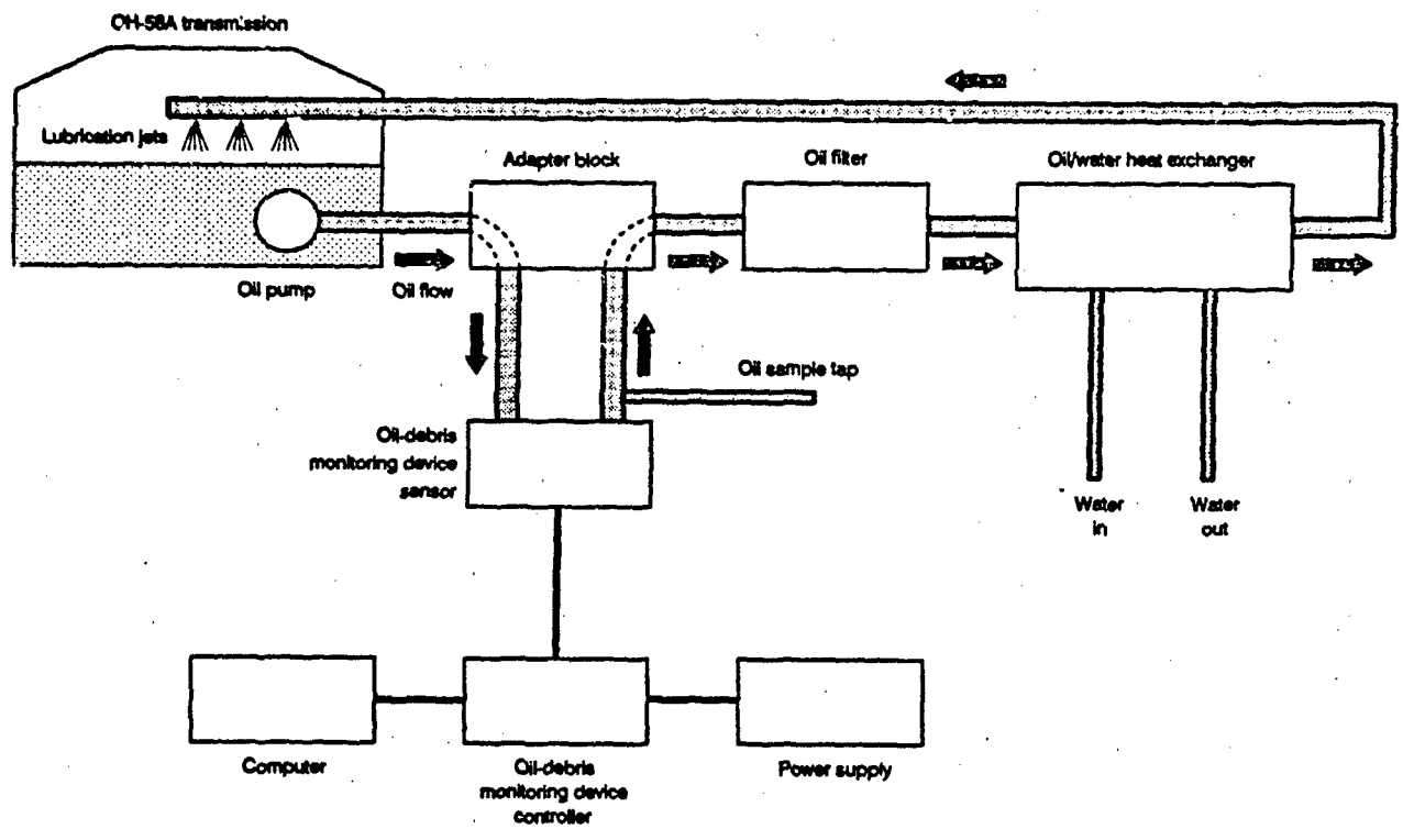
Figure 4. — Transmission lubrication system with oil-debris monitoring device installed.
