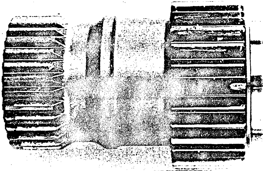
Figure 8. — Spalls on sun gear teeth after test 3.
