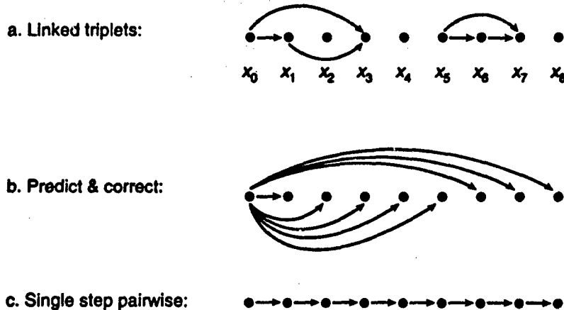
Figure 7. Graphs depicting (a) linked triplets of pairwise estimators, and (b and c) two implementations of the optimal estimator.
