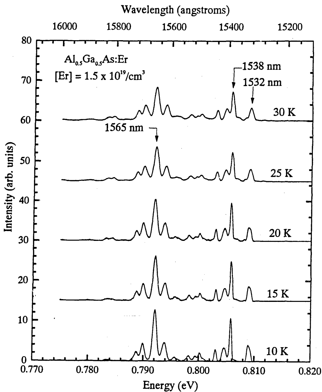
Figure 65 Photoluminescence of MBE grown \text{Al}_{0.5}\text{Ga}_{0.5}\text{As:Er} measured at T = 10, 15, 20, 25, and 30 \text{ K}
