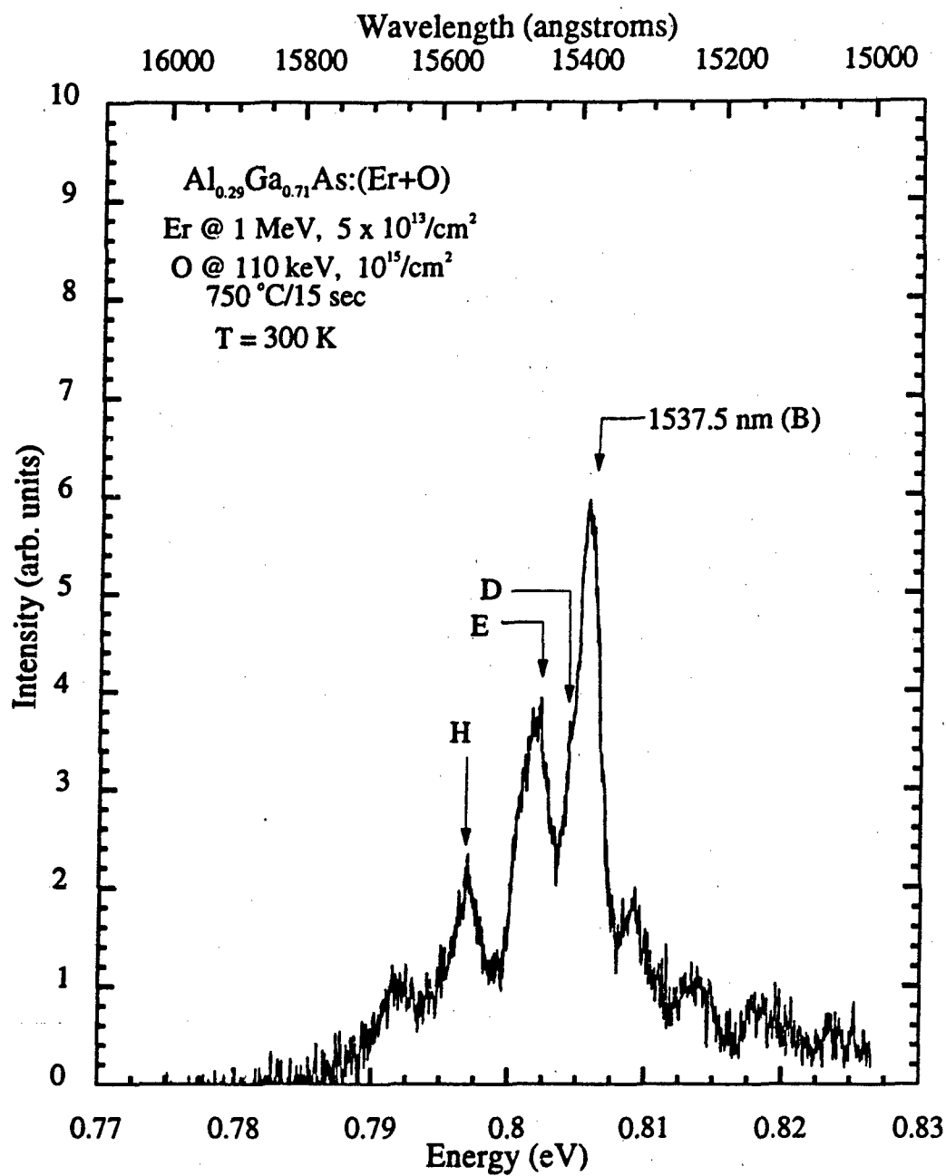
Figure 86 Room temperature photoluminescence from SI-Al 0.29 Ga 0.71 As:(Er+O) implanted with Er at 1 MeV with a dose of 5 \times 10^{13}/\text{cm}^2 and with O at 110 keV with a dose of 10^{15}/\text{cm}^2
