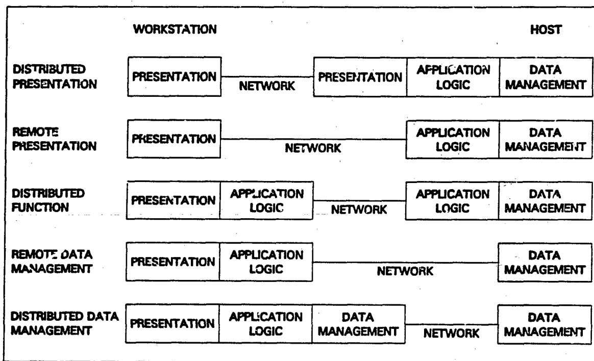
Figure 2-2. Five Basic Client - Server Models
