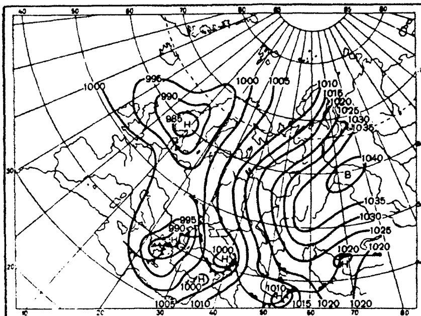
Fig. 11. Weather situation in period of formation of fog on 3 February, 1952.
