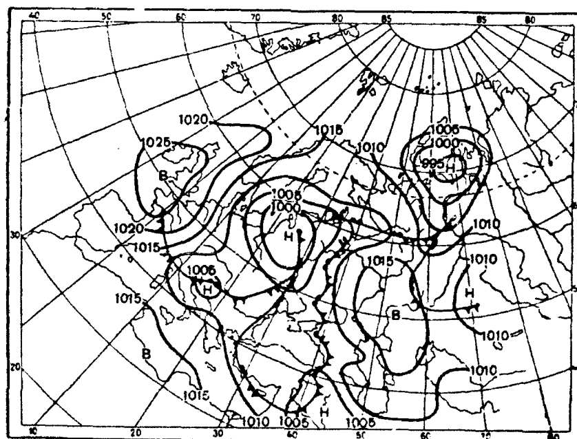
Fig. 23. Weather situation in period of hailstorm in western Georgia on 7 December, 1969.
