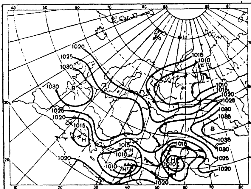
Fig. 12. Weather situation period of formations of fog on 2 January,
