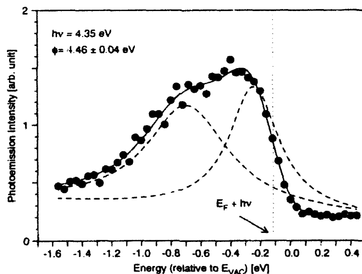
Figure 6. Image potential induced EDC peak on Cu(110) (normal emission, h\nu = 4.35 \text{ eV} ) composed of two broad, image resonances which have blended into a single feature. The E_F + h\nu level has been indicated. The resultant work function is \phi = 4.46 \pm 0.04 \text{ eV} .
