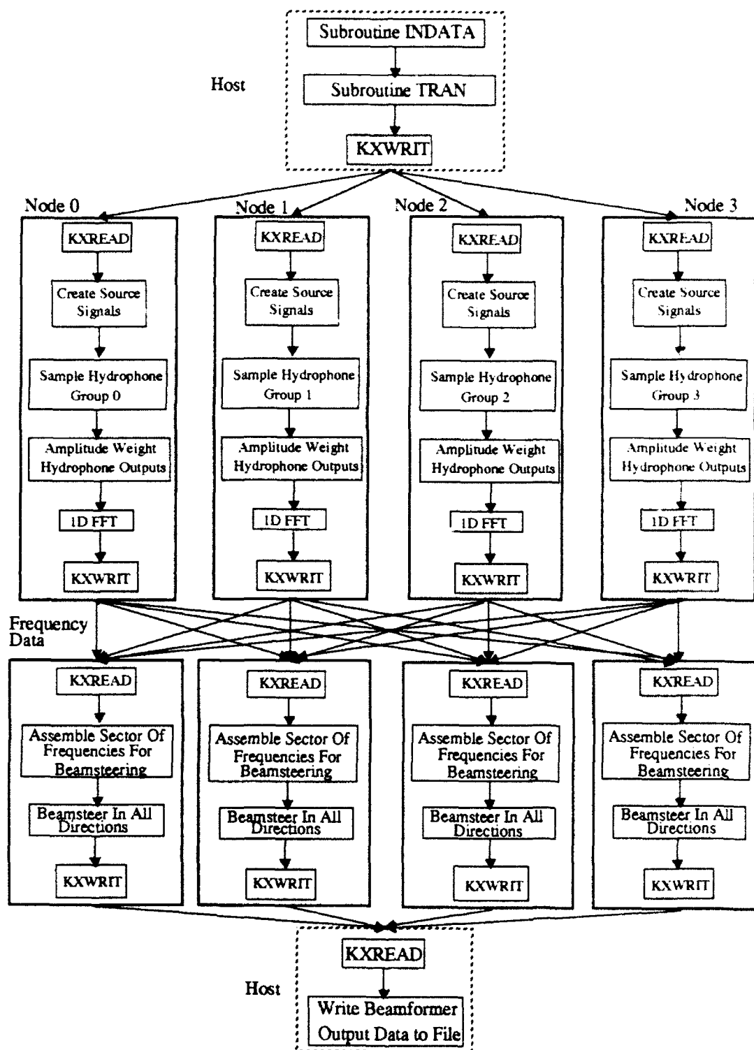
Figure 8.3 Four processor Frequency Partition With Message Shuffle program.
