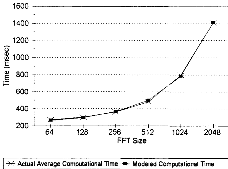
Figure 9.5 Actual and projected processor FFT computation time.
