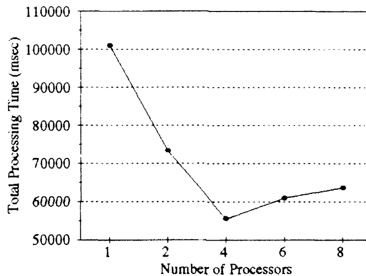
Figure 4.4 Total processing time versus number of processors.
