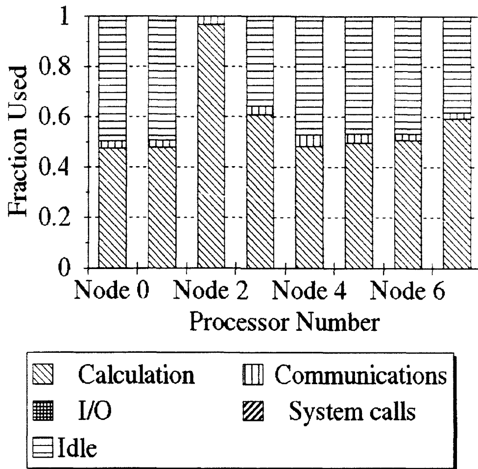
Figure 5.2 Node utilization for eight node Partition Without Message Shuffle method.
