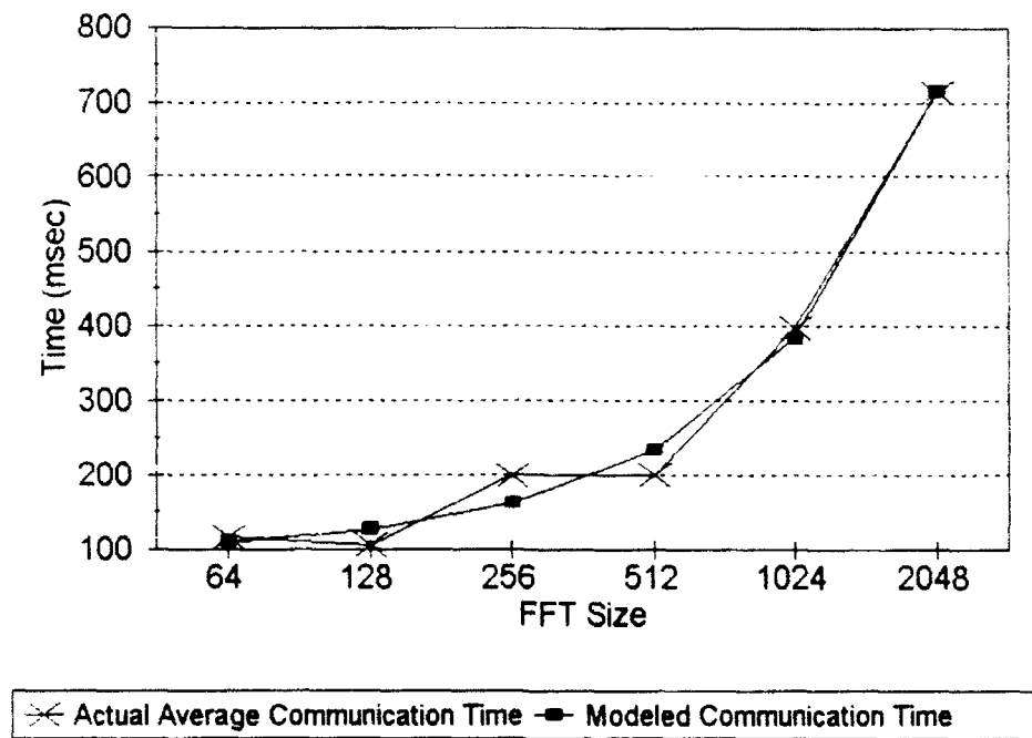
Figure 9.2 Actual and modeled communication time.
