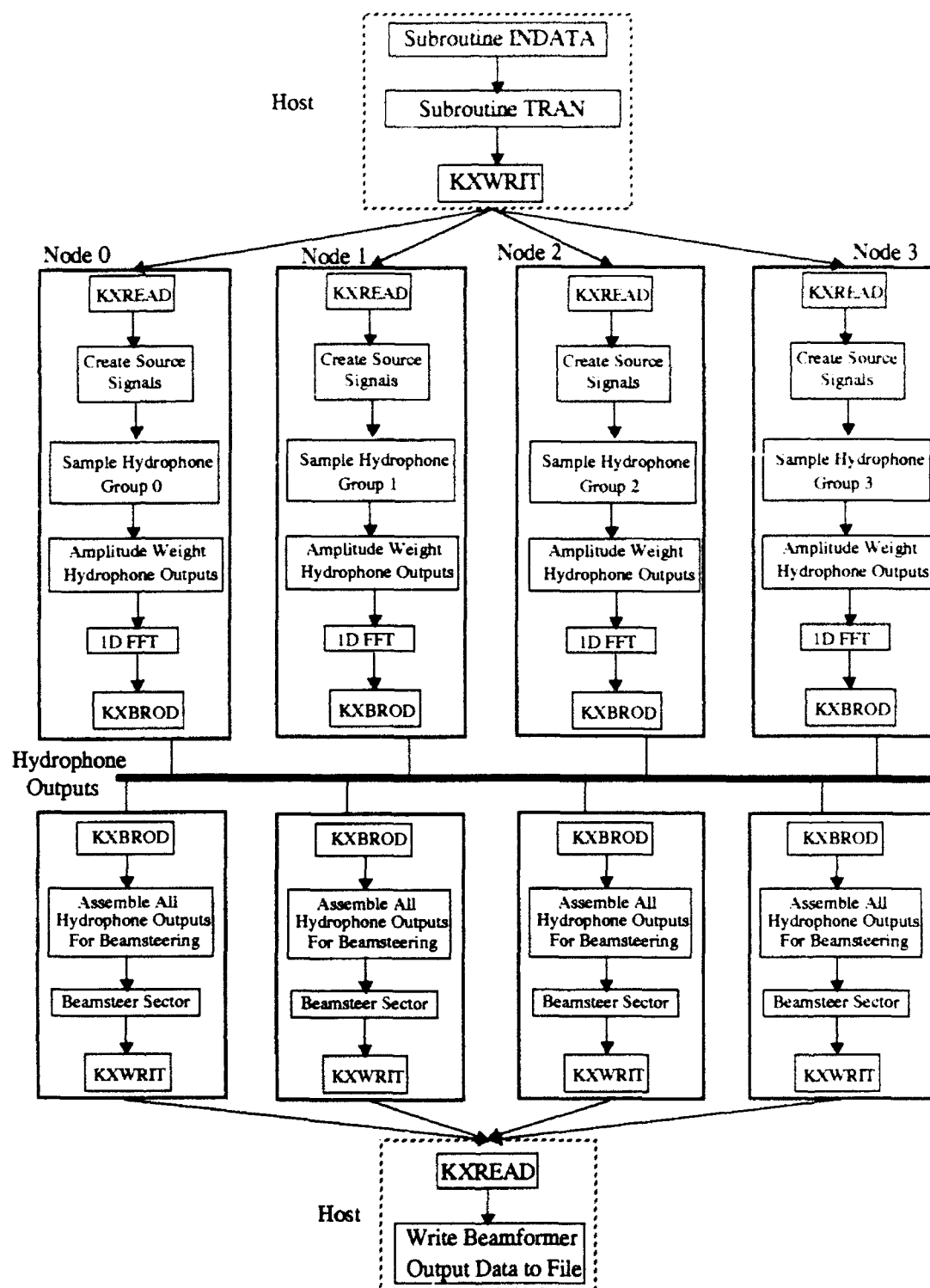
Figure 7.1 Four processor Partition With Message Broadcast program.
