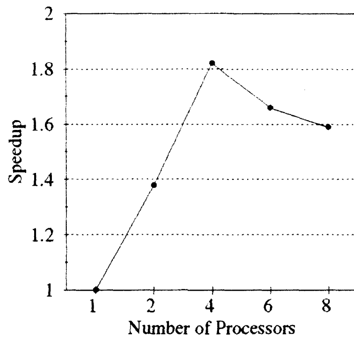
Figure 4.5 Speedup versus number of processors.
