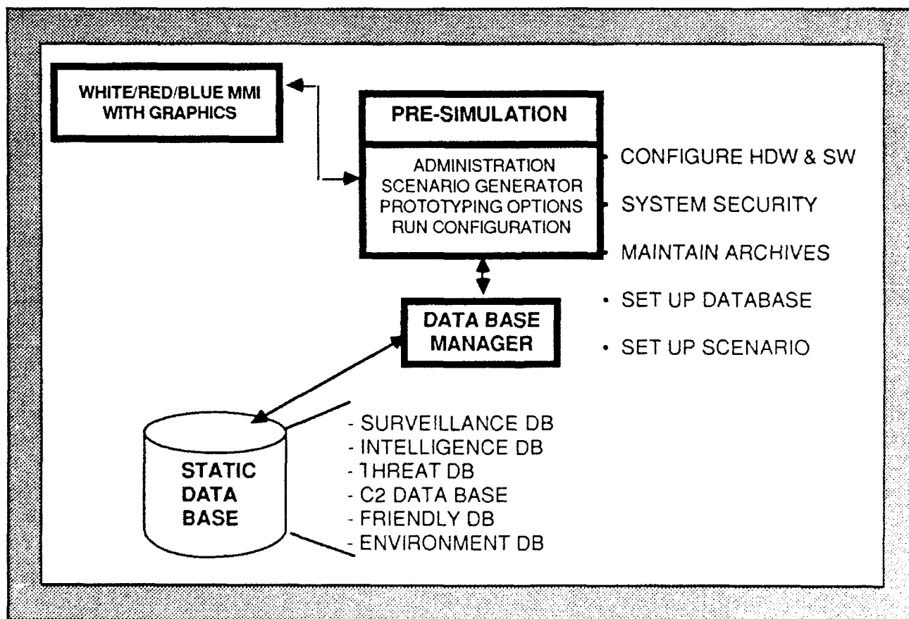
FIGURE 11 - ADISC2 PRE-SIMULATION FUNCTIONAL DESIGN CONCEPT
