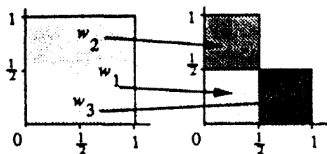
Figure 1. Three affine transformations in the plane.
