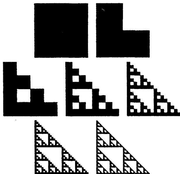
Figure 2. A_0, A_1, A_2, A_3, A_4, A_5 , and A_\infty .
