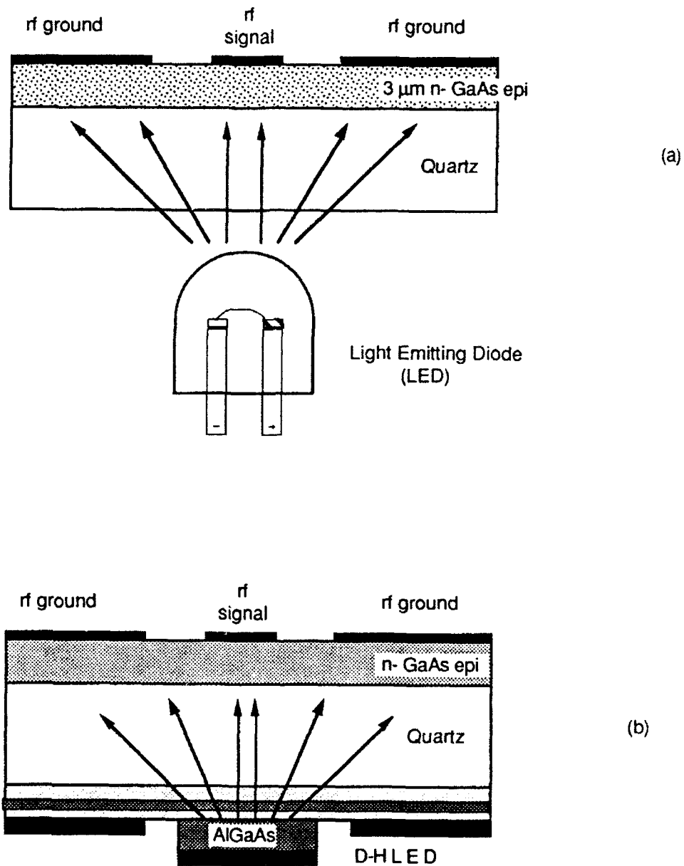
Figure 4: Cross-section of an optically-controlled CPW phase shifter on a GaAs-on-quartz substrate. (a) Configuration of commercially available LED illumination source; (b) Integrated double-heterojunction (D-H) LED/CPW pair using the epitaxial lift-off technique to bond AlGaAs/GaAs layers to both sides of the quartz substrate.
