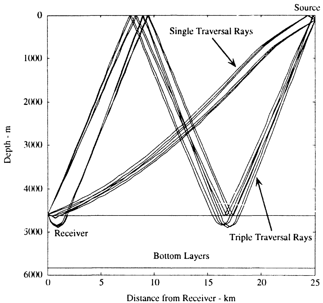
FIG. 1.1 Single and triple traversal rays.
