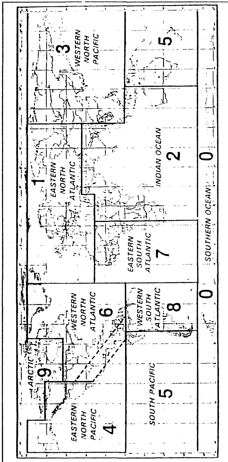
Figure 6 WVS Ocean Basin Areas (DMA, 1988)
