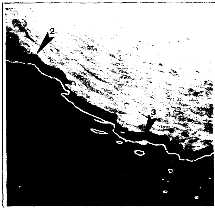
Figure 33 Coastal feature locations before Auto-Avian. (1) Single Island, (2) Simple Coastline and (3) Island-Coast Combination.
