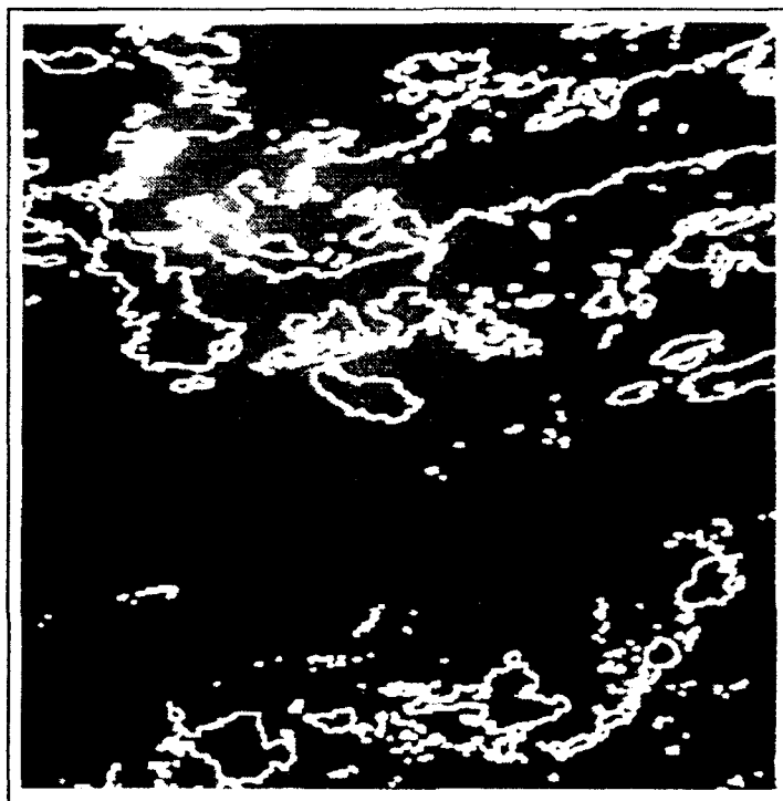
Figure 27 Binary AVHRR (Channel 2) sub-scene (Fig. 26)
