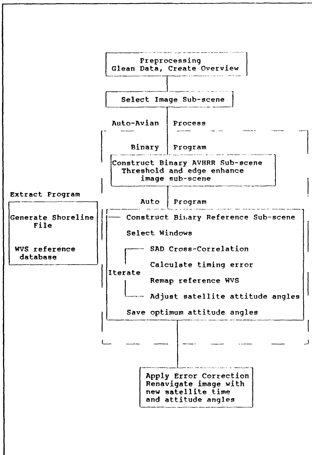
Figure 5 Flowchart of the Auto-Avian method
