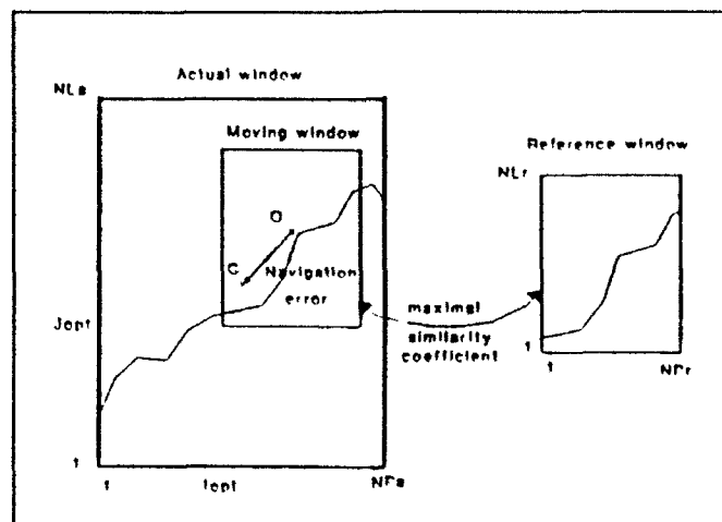
Figure 4 Illustration of navigation error resulting from similarity coefficient adjustment (Bordes et al., 1991)
