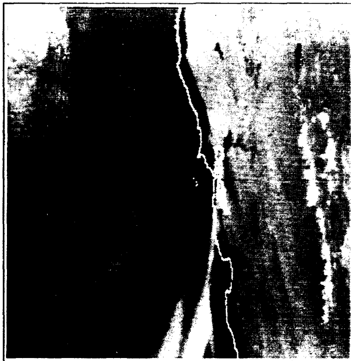
Figure 21 Navigation Error before Auto-Avian method: The WVS depicted in white. Subscene of Fig. 18.
