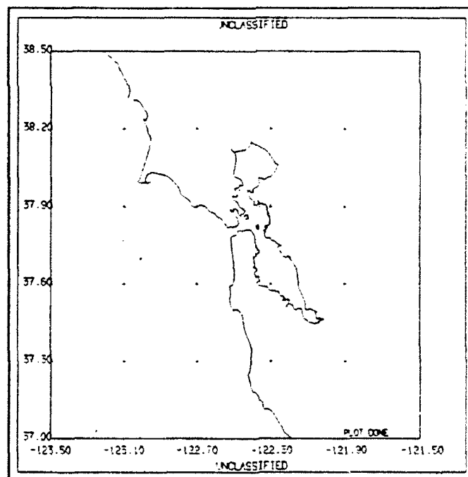
Figure 16 WVS display after reduction (1:500,000 scale)
