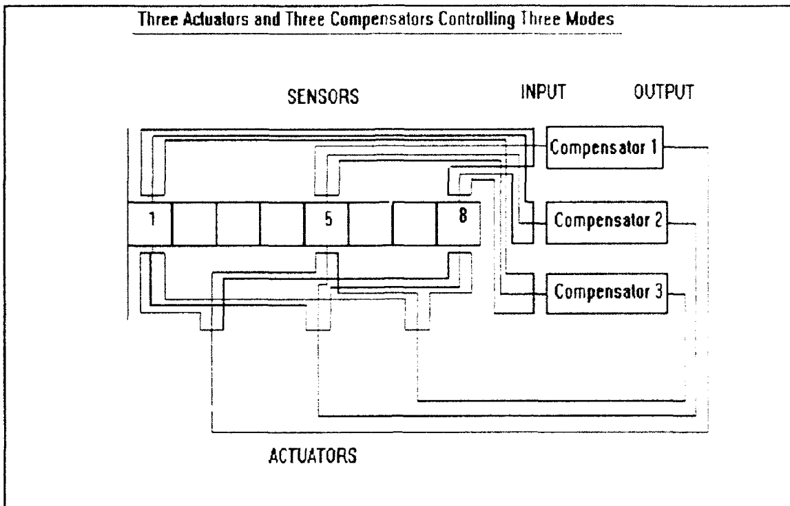
Figure 10 Three Actuator / Three Compensator Control Scheme
