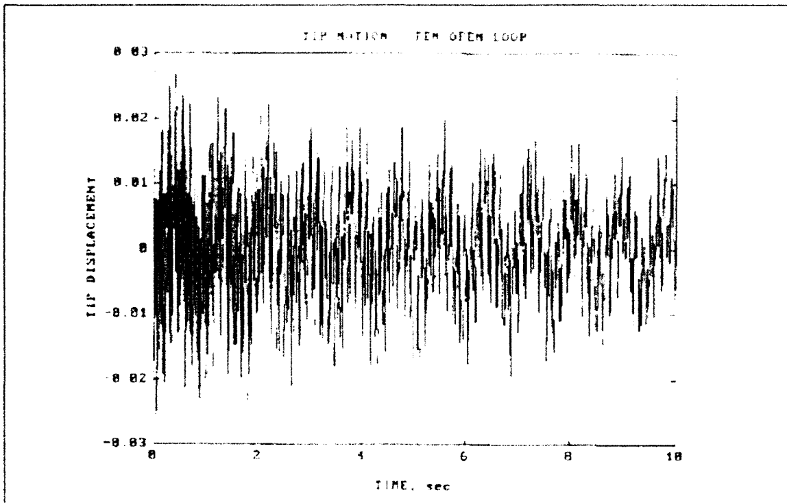
Figure 4 Open-Loop Response
