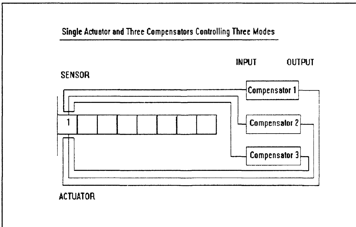
Figure 11 Single Actuator/Three Compensator Control Scheme
