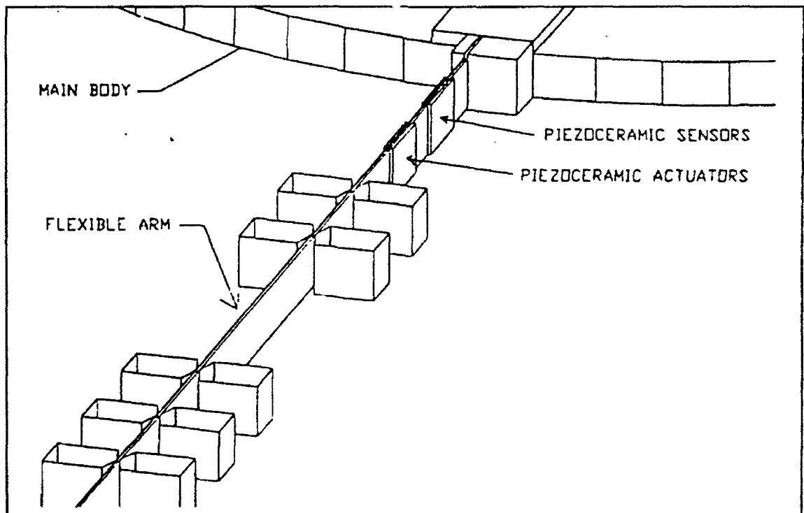
Figure 27 Piezoceramic Locations
