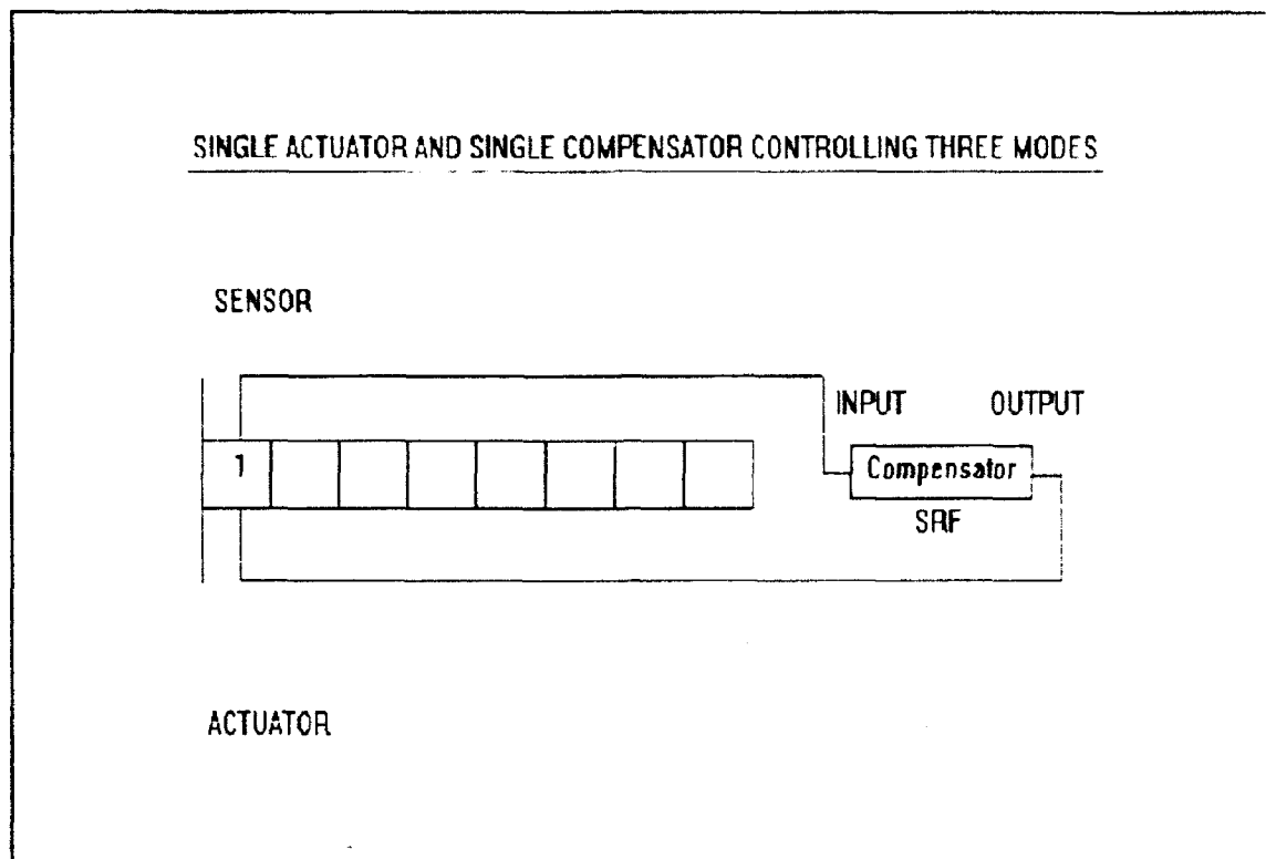
Figure 21 Single Actuator/Single Compensator Control Scheme
