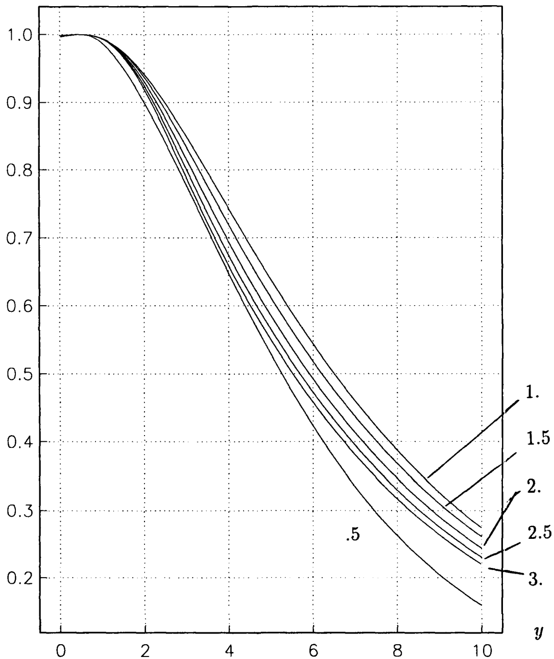
Figure 3.2. The eigenfunction P for different values of the quantity \lambda .
