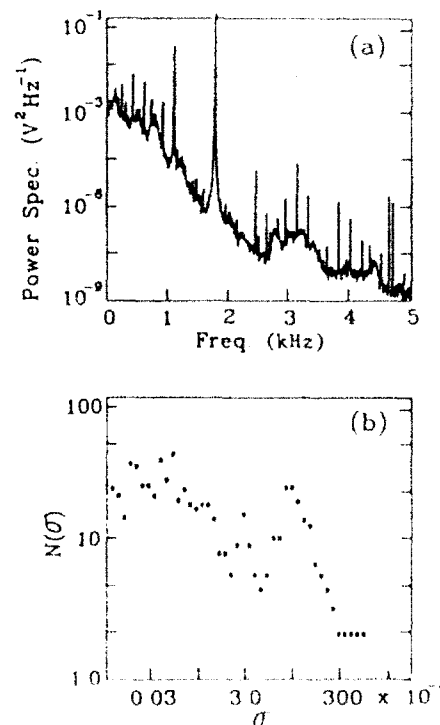
FIG. 6. (a) A power spectrum obtained by analog simulation for the fixed conditions and q_2=0.38 (chaotic), and (b) the threshold dependence of the number of peaks.
