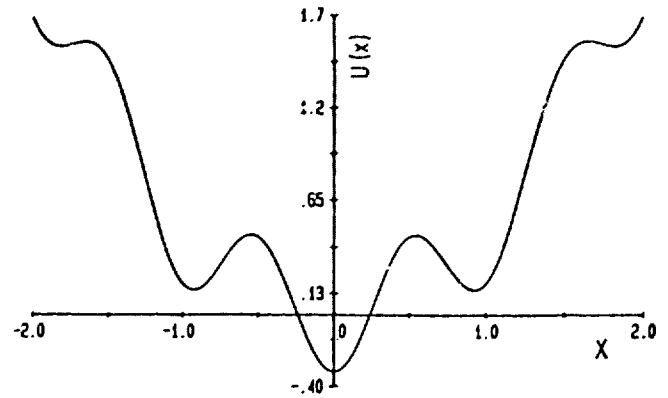
FIG. 1. A Plot of Eq. (4) with \beta = 2 , which was the potential used in this work.
