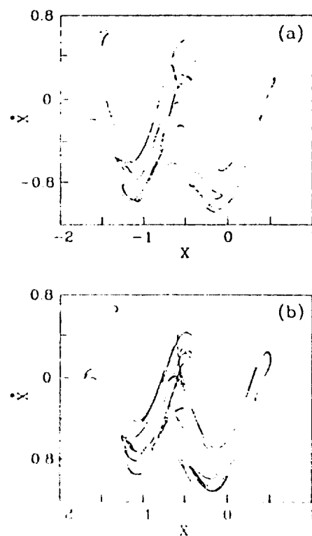
FIG. 3. A SNCA for k = \beta = 2 and q_1 = 2.768 , which are henceforth identified as the "fixed conditions" and with control parameter q_2 = 0.88 , from the dynamics of Eqs. (2)–(4). (a) Measured on the analog simulator with 10 000 points displayed, and (b) obtained by digital simulation for the same conditions with 30 000 points displayed. The Lyapunov exponent, obtained as described in the text, was \lambda = 0.150 for this attractor.
