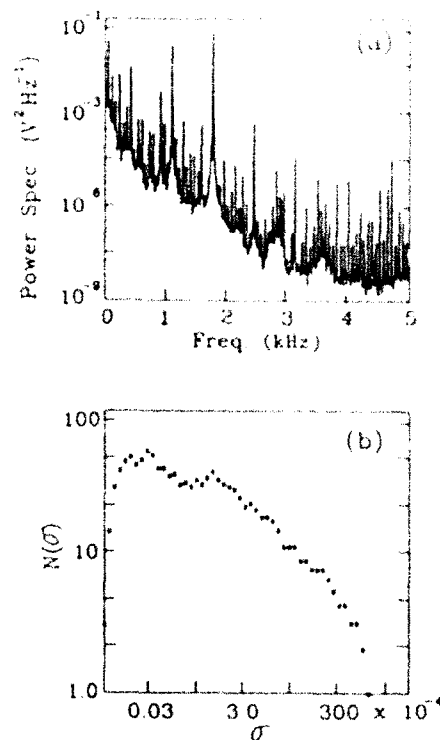
FIG. 5. (a) A power spectrum obtained from the analog simulator for the fixed conditions and q_2=0.88 (SNCA), and (b) the threshold dependence of the number of peaks N(\sigma) with amplitudes greater than the threshold \sigma .
