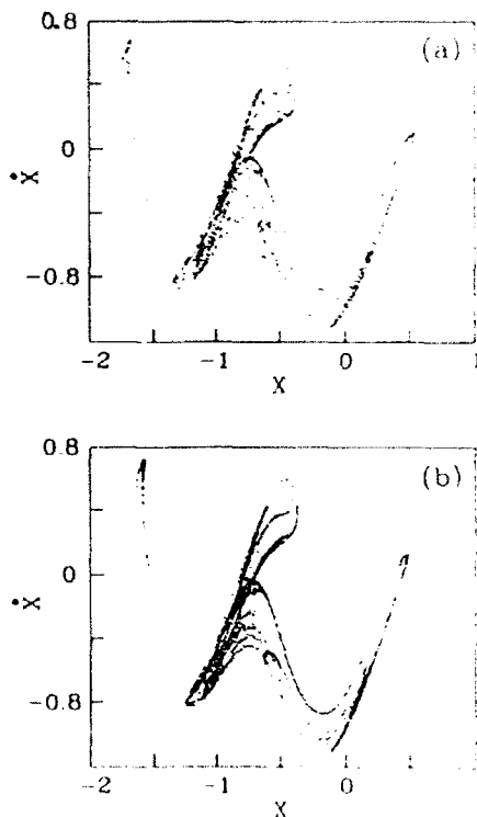
FIG. 4. A chaotic attractor for the fixed conditions with q_2=0.38 . (a) Measured on the analog simulator ( 10^4 points), and (b) by digital simulation ( 3 \times 10^4 points) from which \lambda=0.156 was obtained.
