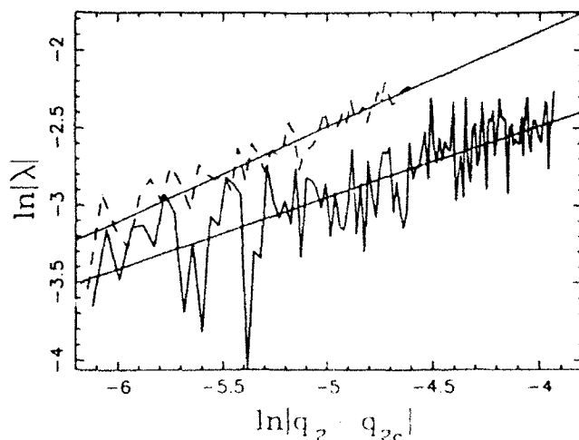
FIG. 8. The Lyapunov exponent as an order parameter in the destruction of chaos by a SNCA. The results for the chaotic attractor are shown by the dash-dotted line, and for the SNCA by the solid line. The straight lines are least-squares fits to the data and have slopes 0.613 and 0.463 for the chaotic and nonchaotic attractors, respectively.
