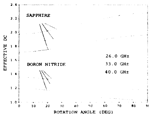
Fig. 4. Effective dielectric constant versus \theta of the bilateral fin-line on boron nitride and sapphire with a = 7.112 mm, b = 3.556 mm, h_1 = 0.0625 mm, h_2 = 3.4935 mm, w = 0.5 mm.
