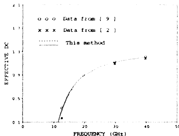
Fig. 2. Effective dielectric constant of the bilateral fin-line with a = 7.112 mm, b = 3.556 mm, h_1 = 0.0625 mm, h_2 = 3.4935 mm, w = 0.5 mm on isotropic substrate with \epsilon_1 = \epsilon_2 = \epsilon_3 = 3.75 and \mu_1 = \mu_2 = \mu_3 = 1.0 , and dielectrically uniaxial substrate with \epsilon_1 = \epsilon_3 = 3.0 , \epsilon_2 = 3.5 , and \mu_1 = \mu_2 = \mu_3 = 1.0 .
