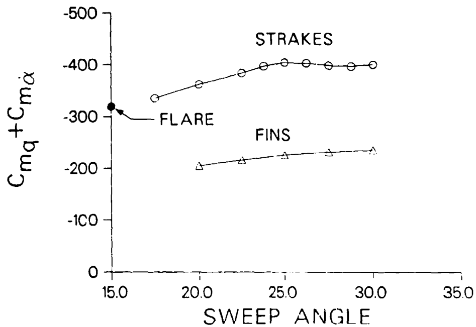
Figure 36. Pitch damping moment coefficient, Scorpion configurations, computation vs sweep angle of fins and strakes
