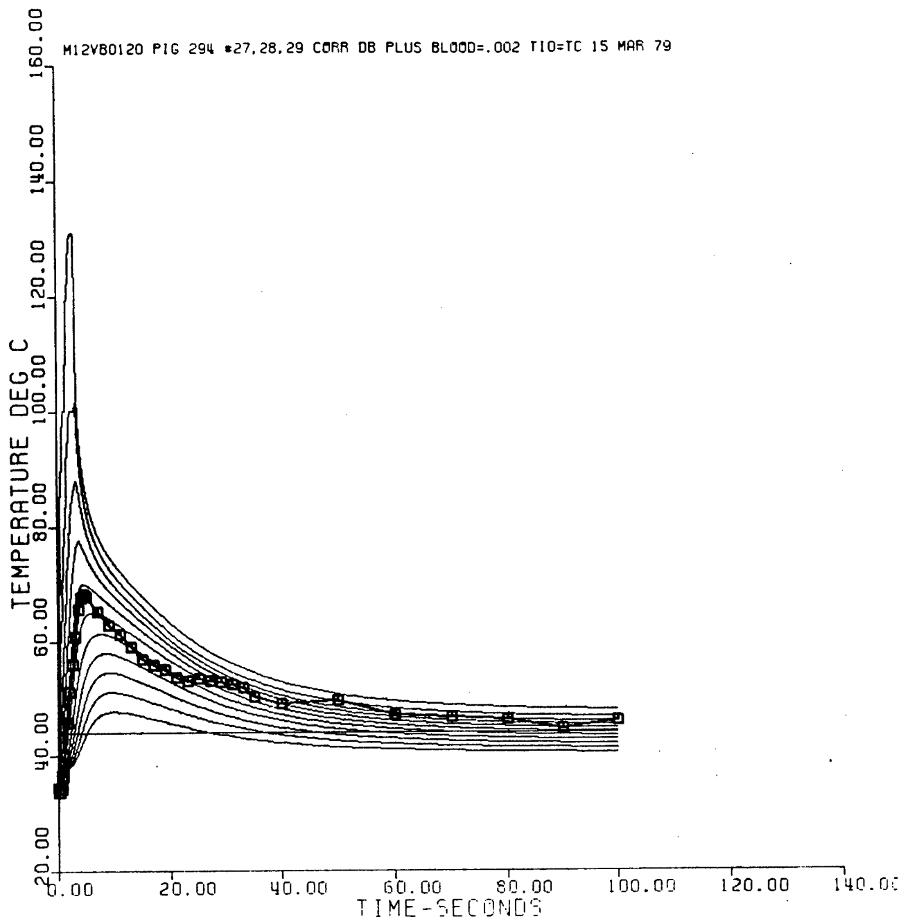
Figure A-6. Predicated skin temperature at each node (solid lines) and measured intraskin temperature in pig 284 location #29 when exposed to 3.47 \text{ cal} \cdot \text{cm}^{-2} \cdot \text{sec}^{-1} for 3.02 seconds
