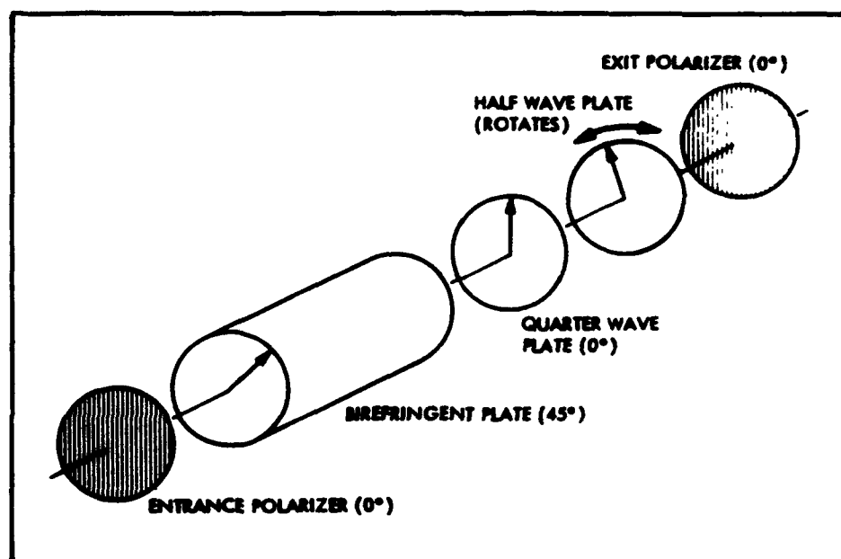
Figure 3.6: Birefringent tuning element. From Title & Rosenberg (1981).
