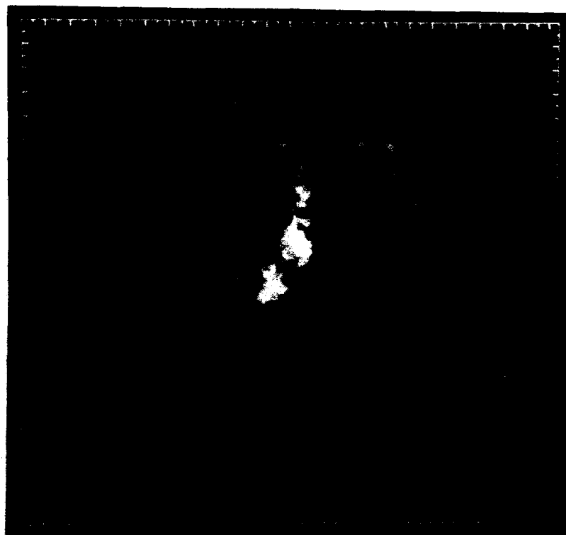
Figure 6.1: Magnetogram of AR6181. The three outlined subfields were used separately to measure wave properties in network field and quiet regions. The small tick marks are 5".
