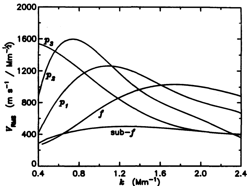
Figure 7.4: RMS velocity vs. k . Curves fitted from quiet subfield velocity spectrum. Curve labeled sub- f is taken from the background fit.
