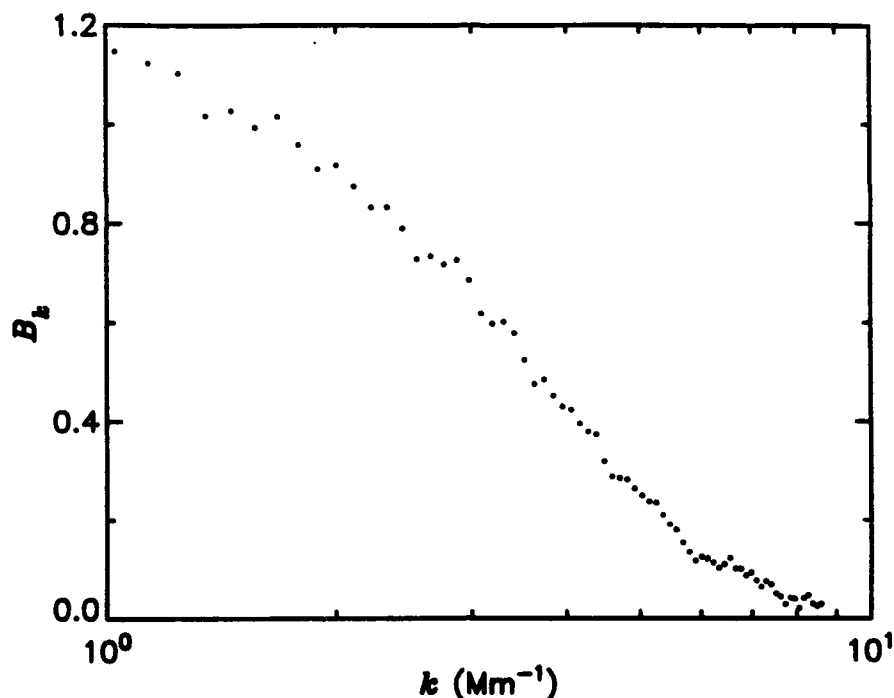
Figure 6.6: Power law exponent for background fit. Exponent vs. wavenumber.
