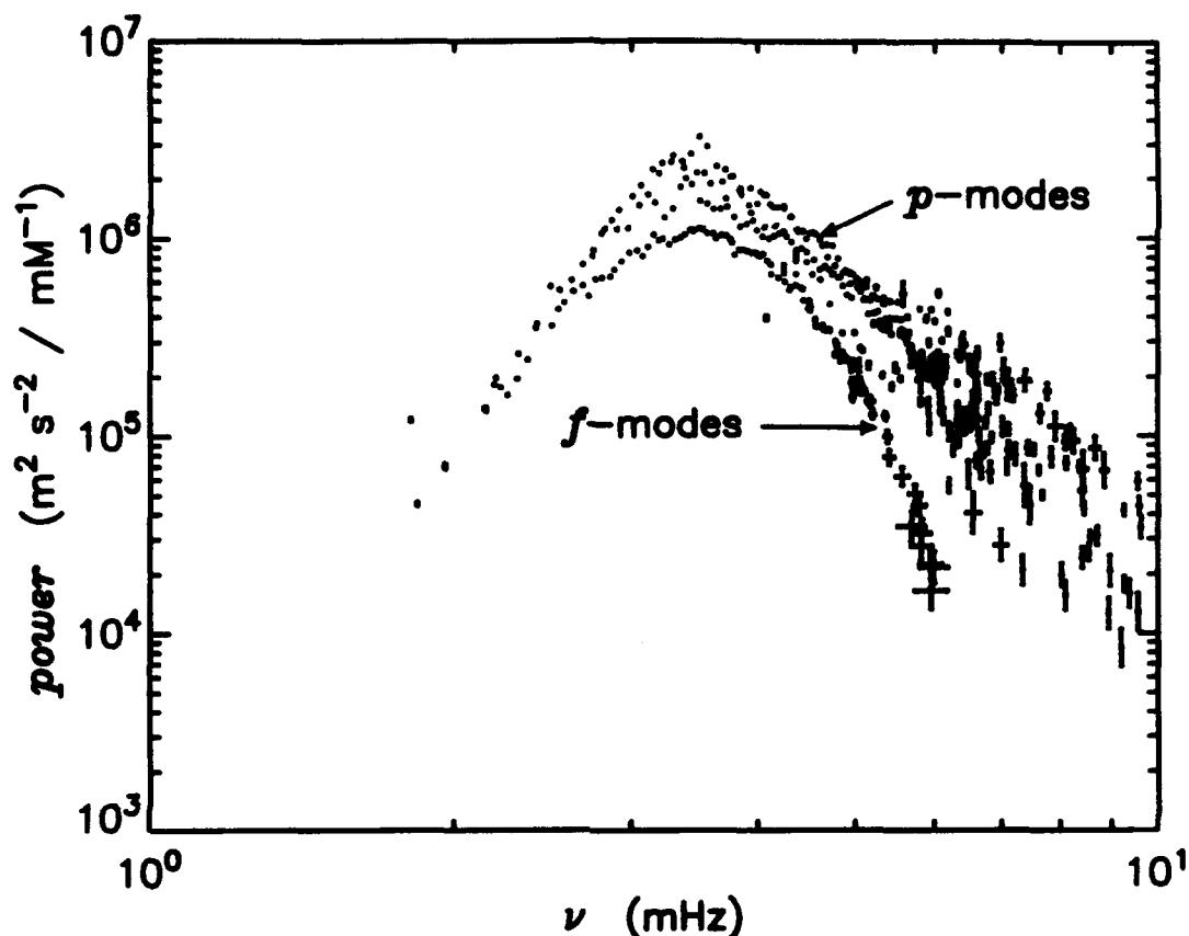
Figure 6.15: Velocity power vs. mode frequency. From Fernandes et al. (1992).
