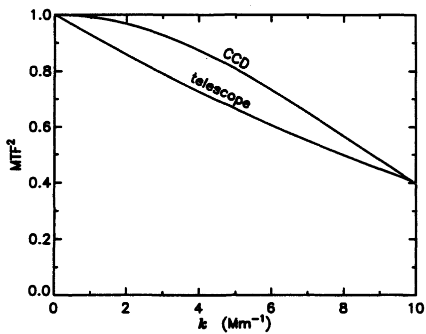
Figure 3.12: Squared MTF of telescope and CCD detector
