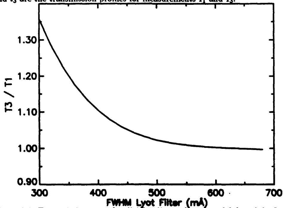
Figure 2.6: Transmission ratio \int t_3 d\lambda / \int t_1 d\lambda as a function of fwhm of the Lyot filter.
