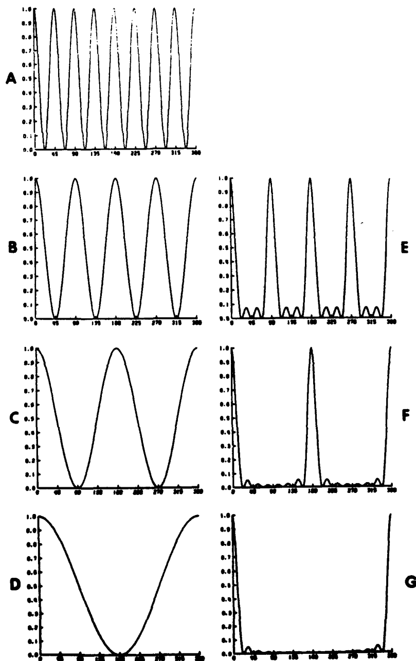
Figure 3.5: Transmission vs. frequency for the components of a Lyot filter (A, B, C, D) and the transmission through successive stages of the cascade (E, F, G). From Title & Rosenberg (1981).
