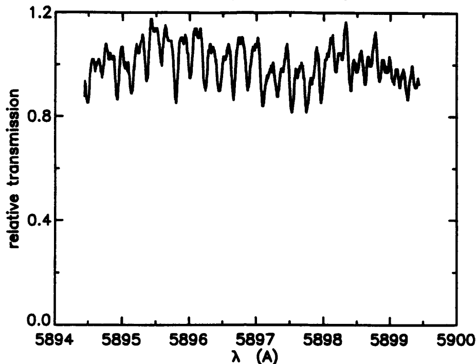
Figure 3.8: Relative transmission of the SOUP tunable filter vs. tuned wavelength. Transmission was measured using a continuum illumination source.
