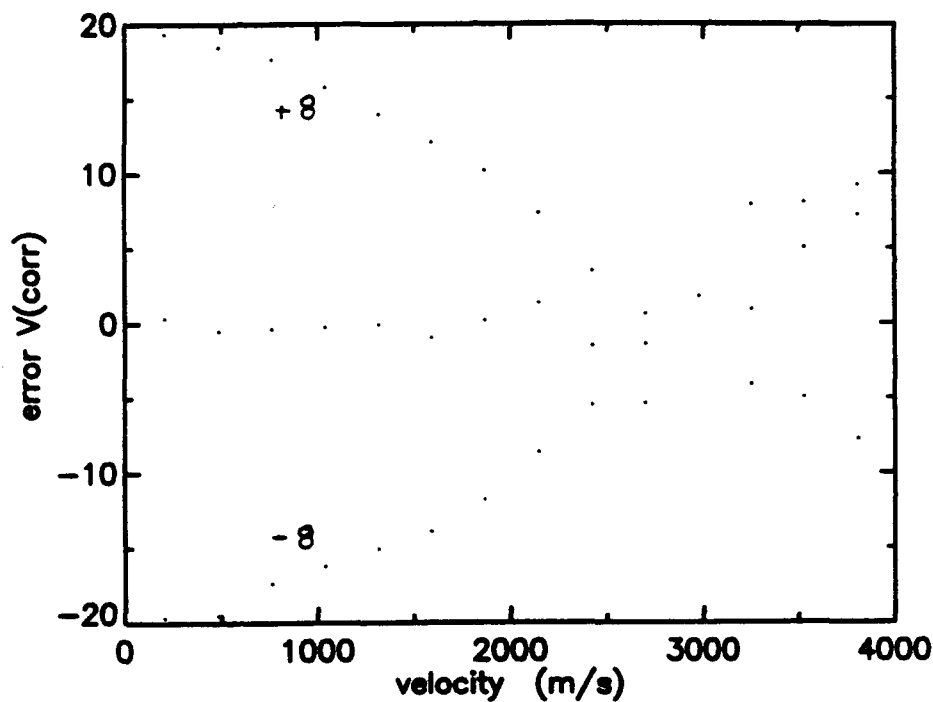
Figure 2.8: Systematic error \epsilon_v vs. velocity for Lyot drifts: -8, 0, 8 mÅ.
