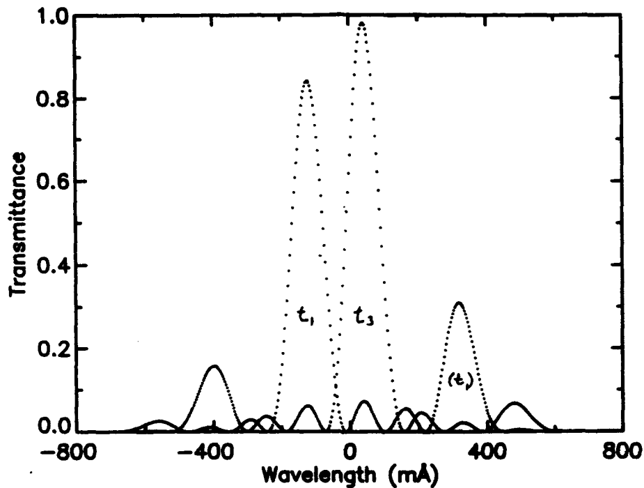
Figure 2.5: Transmission product for Lyot and Michelson filters vs. wavelength. t_1 and t_3 are the transmission profiles for measurements I_1 and I_3 .
