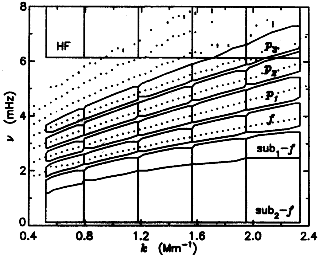
Figure 7.1: Masks for power distribution maps. Measured mode frequencies are shown as dots. Mask limits are shown as solid lines. The high frequency (HF) masks covered the range 6.0 < \nu/\text{mHz} < 10.0 ; the p -mode mask limits were set halfway between modes; the f -mode limits were set equidistant from the f -mode; the \text{sub}_2-f band extends from the f -mode down to \nu = 0 ; the \text{sub}_1-f band is the same width as the f -mode band. It is a subset of the \text{sub}_2-f band.
