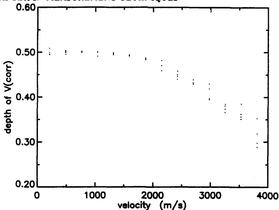
Figure 2.13: Depth of measured velocity vs. velocity for bisector shape hwhm : -7.5, \dots, 7.5 \text{ m}\text{\AA} ( \alpha, \beta method)
