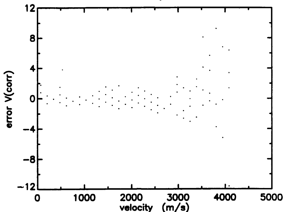
Figure 2.10: Systematic error \epsilon_v vs. velocity for line-width increments: 0, 10, 20, 30% ( \alpha , \beta method).
