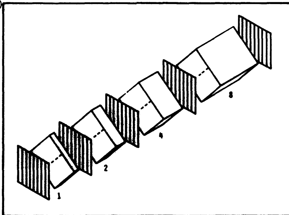
Figure 3.4: Lyot filter with four elements. From Title & Rosenberg (1981).
