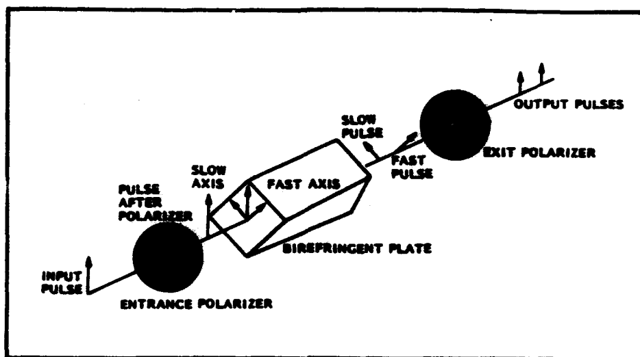
Figure 3.3: Pulse propagation through a simple element. From Title & Rosenberg (1981)
