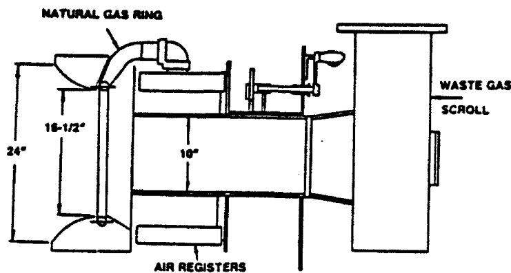
Figure 12. Existing burners.
