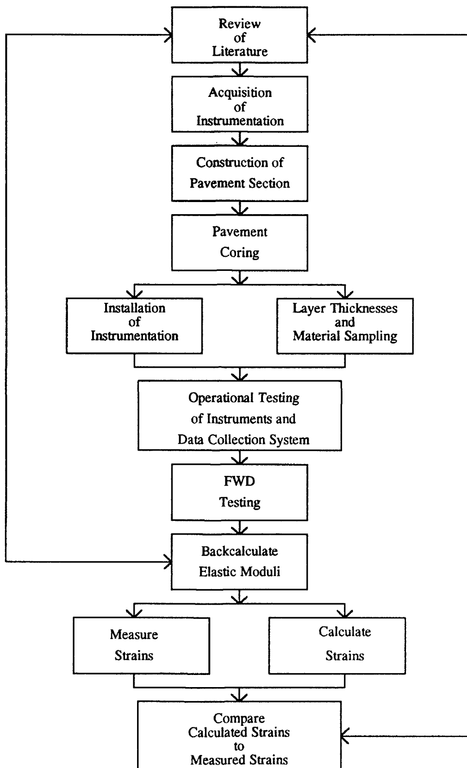
Figure 1. Instrumentation and Initial Evaluation of Test Section
