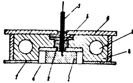
Fig. 3 Anode structural diagram. 1 - anode strip, 2 - ceramic plate, 3 - wire lead, 4 - aluminum oxide powder, 5 - epoxy resin, 6 - glass plate, 7 - ceramic plate, 8 - anodized aluminum plate, 9 - cooling passage.
