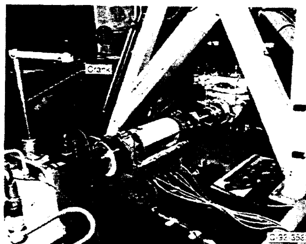
Figure 10.—Setup for static stress tests.
