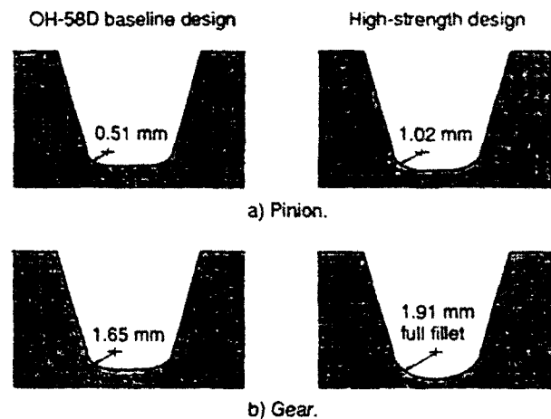
Figure 2.—Comparison of OH-58D and high-strength spiral-bevel gear designs.
