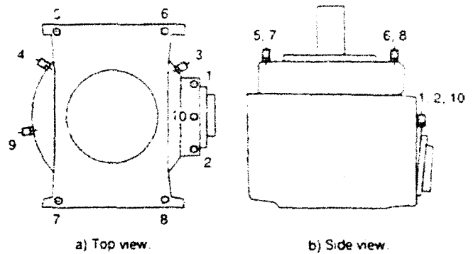
Figure 6.—Accelerometer locations on OH-58D transmission.
