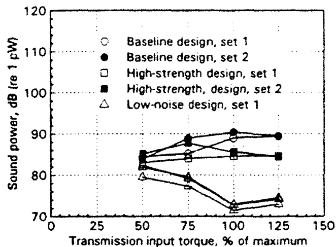
Figure 12.—Noise test results; sound power at spiral-bevel mesh frequencies (first two harmonics) versus transmission input torque.
