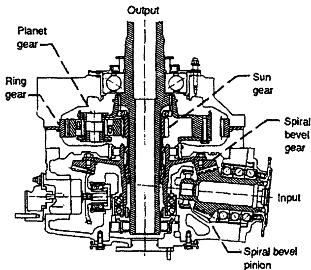
Figure 1.—OH-58D helicopter main-rotor transmission.
