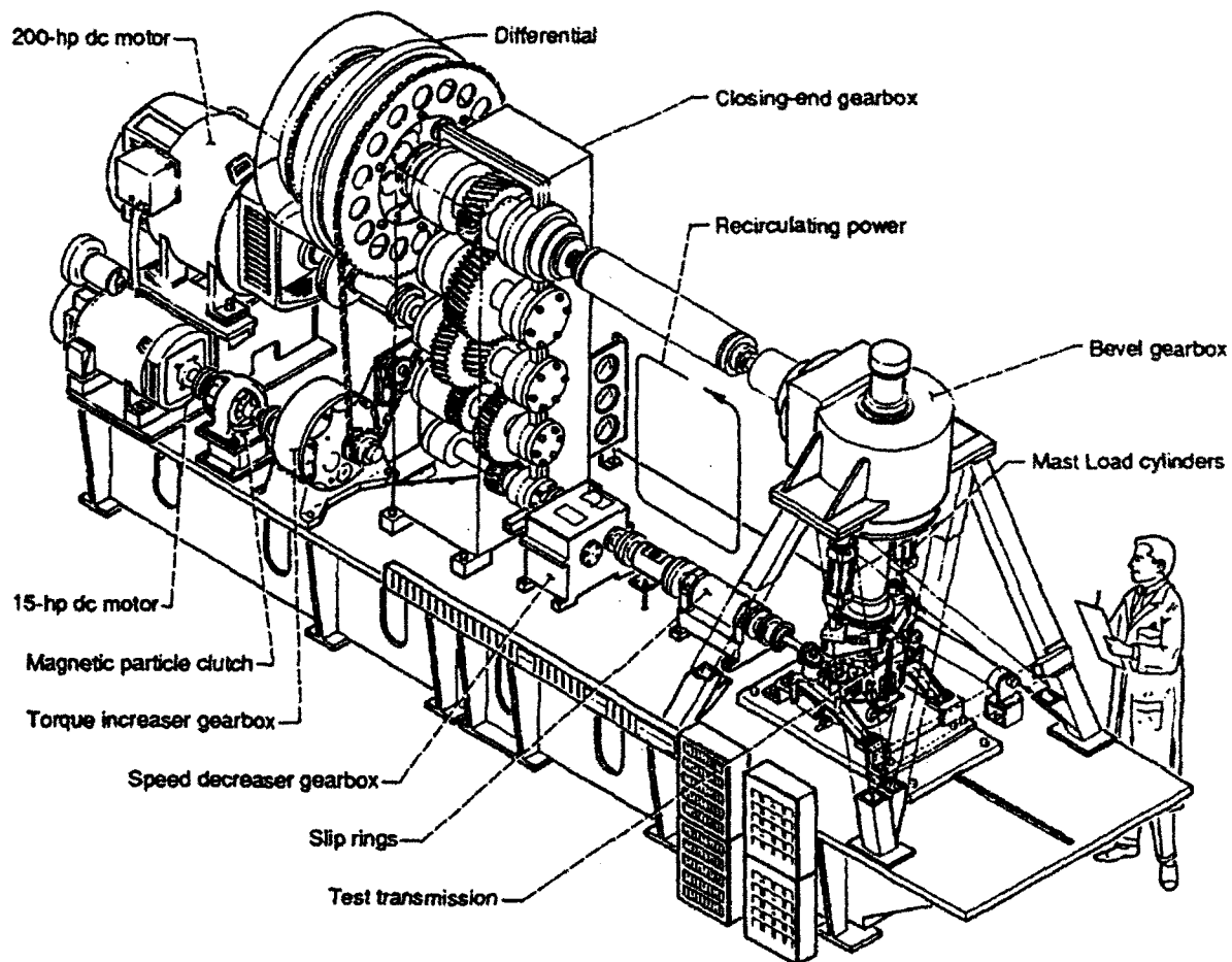
Figure 4.—NASA Lewis 500-hp helicopter transmission test stand.
