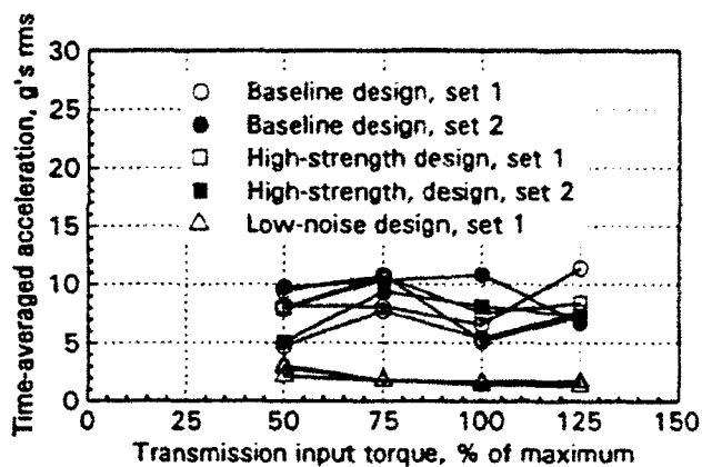
a) Accelerometer 1, input spiral-bevel housing.
