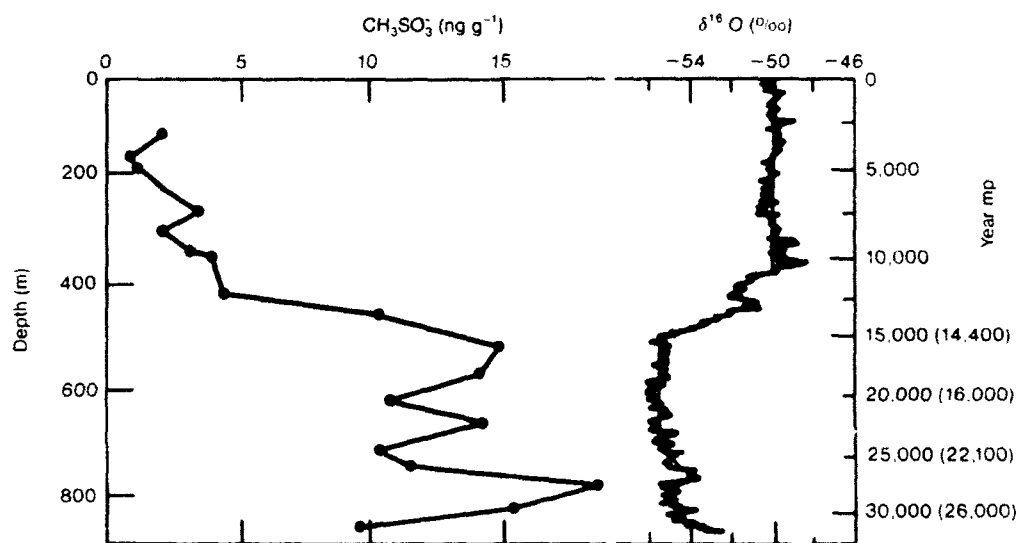
Figure 6. MSA ( \text{CH}_3\text{SO}_3 ) down the Dome C core; the isotope profile ( \delta\text{D}^{\text{O}}/\text{oo} ) indicate the Holocene and the end of the last ice age.
