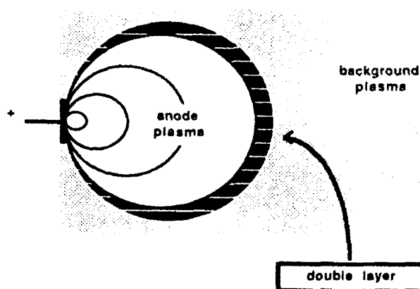
Fig. 10. When the applied potential is too high for quasi-neutrality to be maintained throughout the plasma, a localized nonneutral region known as a double layer forms. The anode plasma can be created by the plasma source or by sheath ionization.
