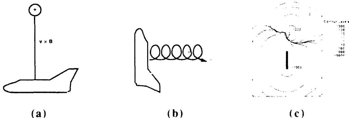
Fig. 2. (a) The operation of an electrodynamic tether. (b) the emission of particle beams, and (c) the biasing of exposed spacecraft surfaces are processes that actively charge spacecraft.
