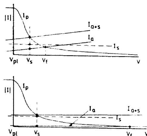
Fig. 1. Simplified current-voltage characteristics of a spacecraft, showing the effect of active ion emission in dense (top panel) and tenuous (bottom panel) plasma. V_f ... floating potential for I_s=0 , V_s ... potential with ion emission, I_a , I_p , I_s ... ambient electron, photo-electron, and ion source currents.
