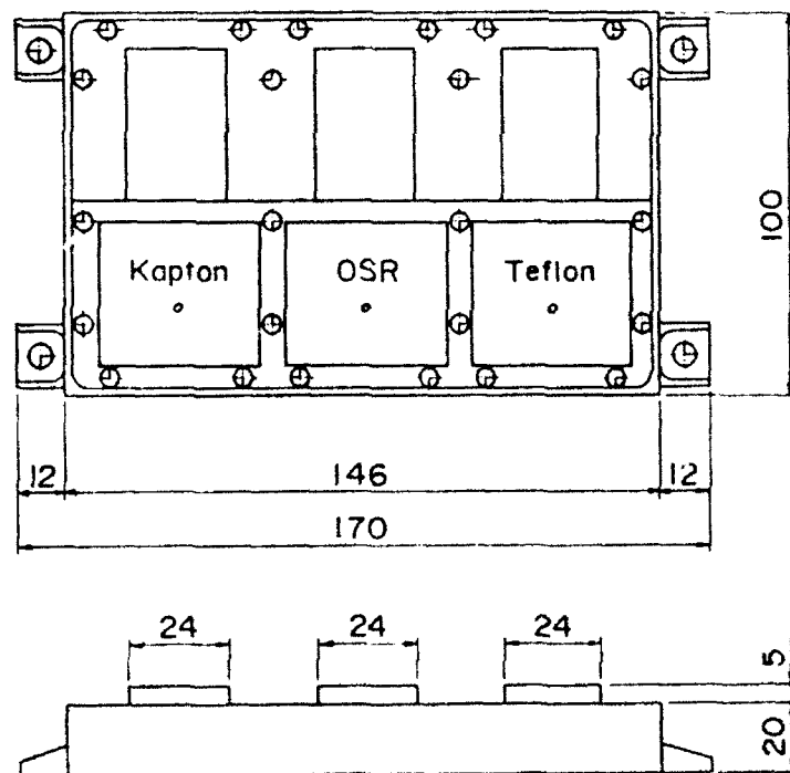
Fig.2 External dimension of POM-S installed on ETS-V.
