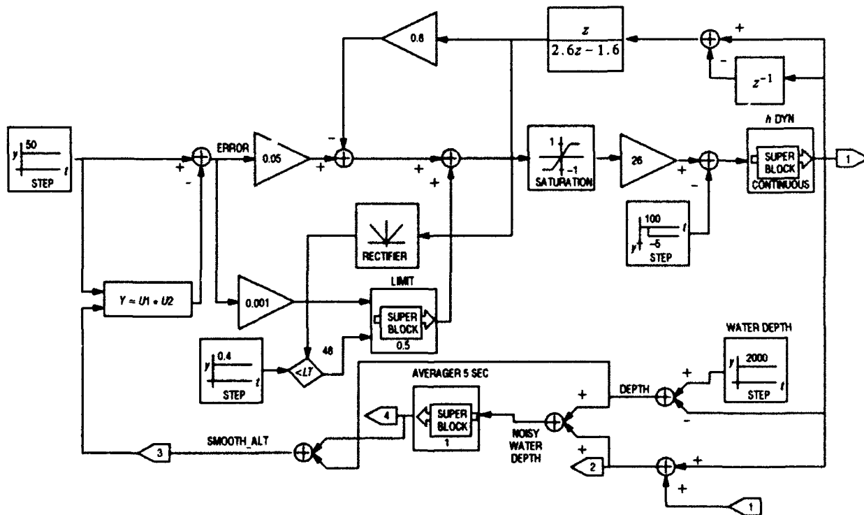
Figure 19. Hover altitude simulation.
