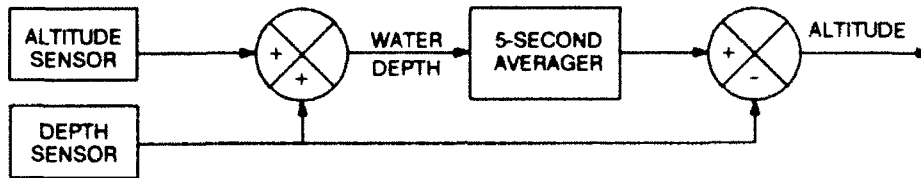
Figure 17. Altitude filter.
