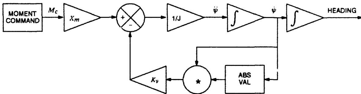
Figure 1. Hover heading.
