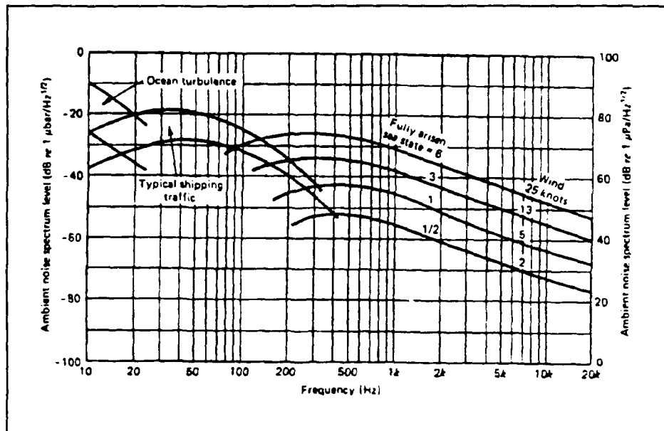
Figure 30: "Wentz" Ambient Sea Noise Curves
