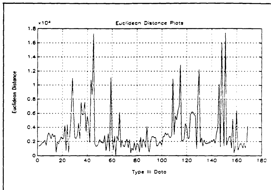
Figure 8: Euclidean Distance for Type III Data
