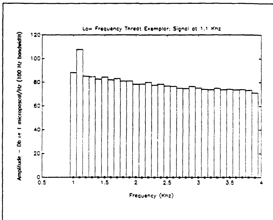
Figure 31: LF Threat Exemplar; Band Level Processed
