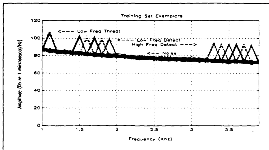
Figure 33: Entire Training Data Set
