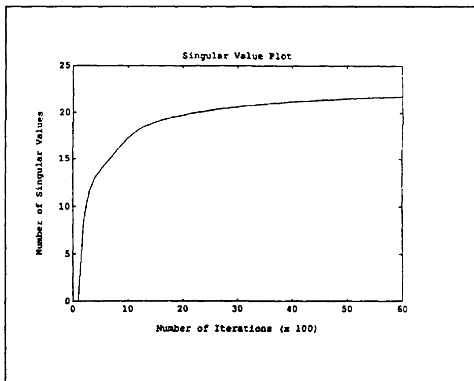
Figure 9: Singular Value Decomposition
