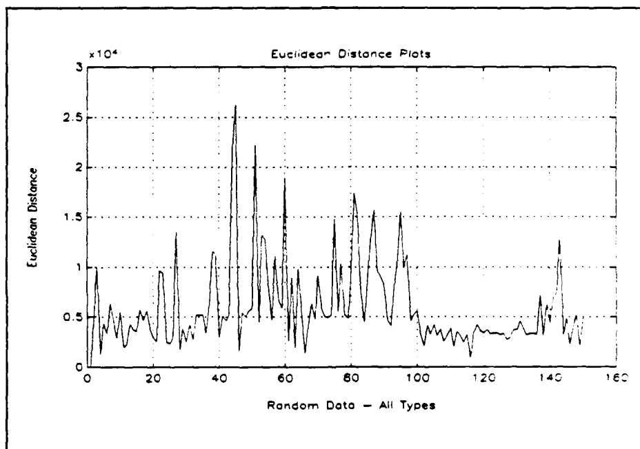
Figure 5: Euclidean Distance for all Data Types
