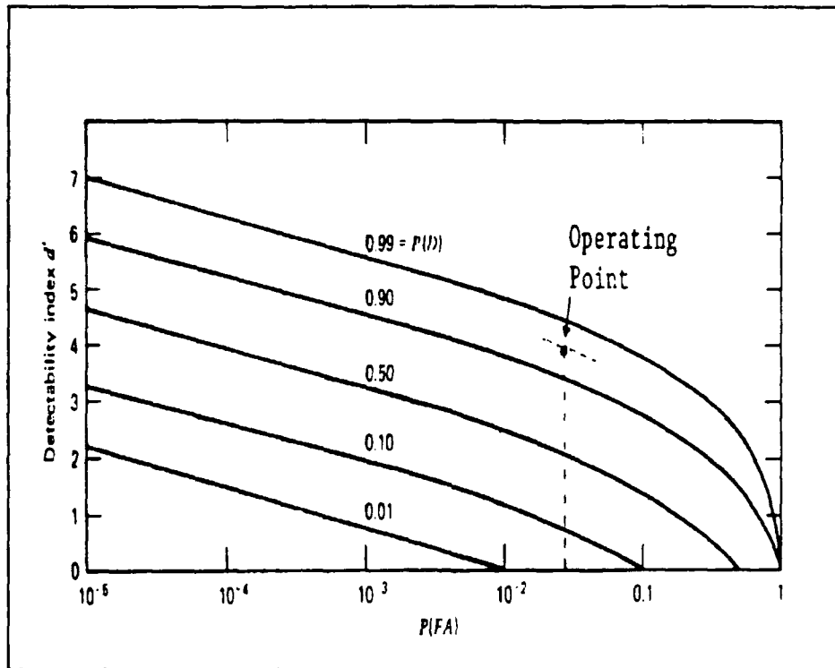
Figure 29: Detectability Index Curves
