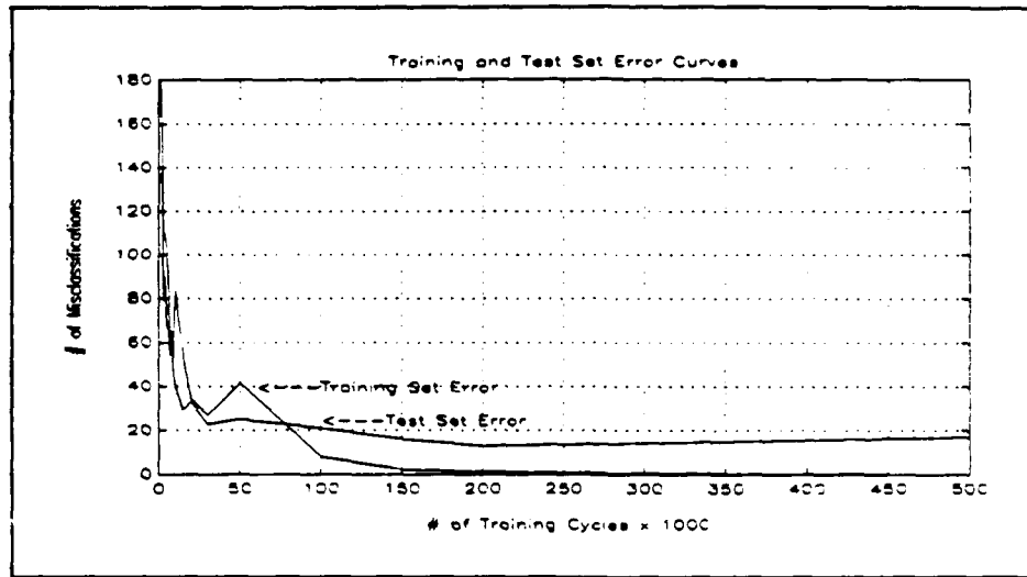
Figure 10: Optimum Network Training Time
