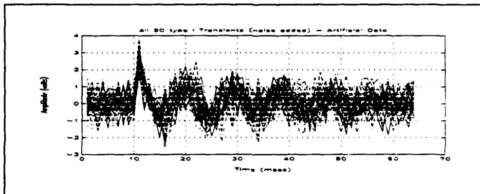
Figure 19: All Type I Transients with Noise Added
