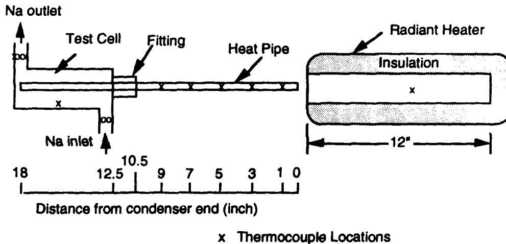
Figure 5.1: Experimental setup
