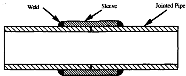
Figure 3.1: A Typical Sleeve Weld.
