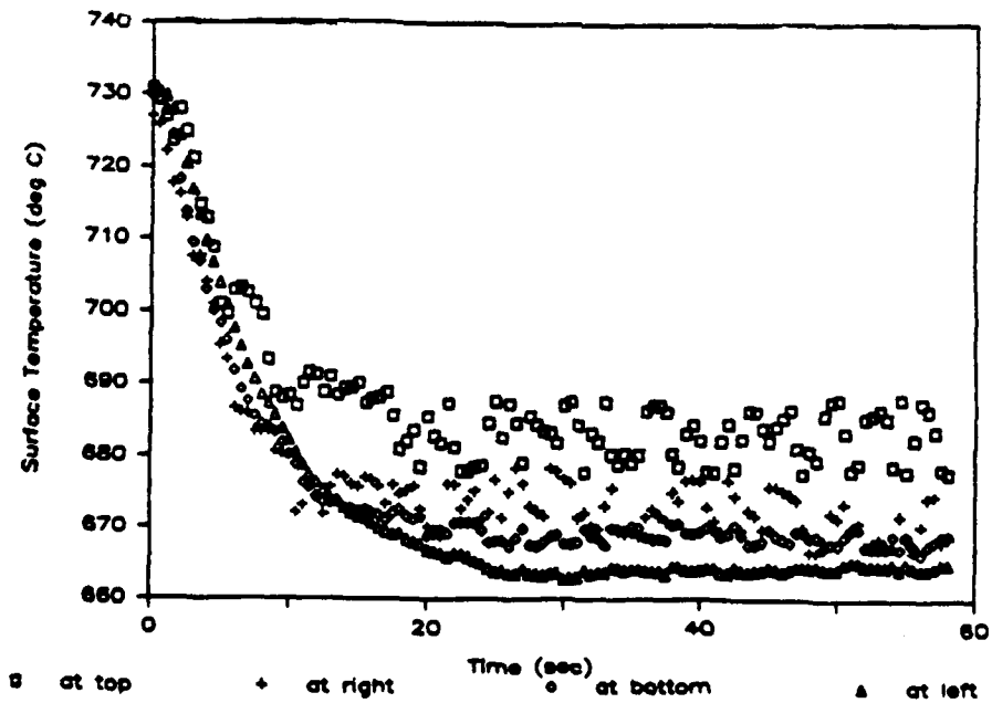
Figure 5.7c: Circumferential Surface Temperature
