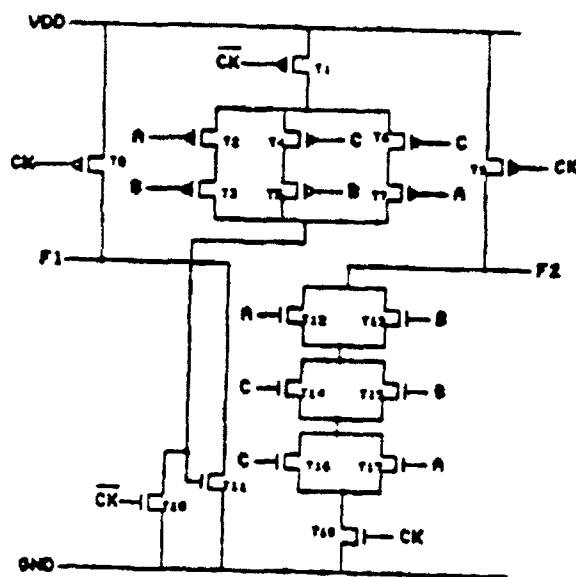
FIG. 9 TOTALLY SELF-CHECKING CMOS CIRCUIT REALIZING FUNCTION F_1 = A + B + C AND F_2 = A + B + C
