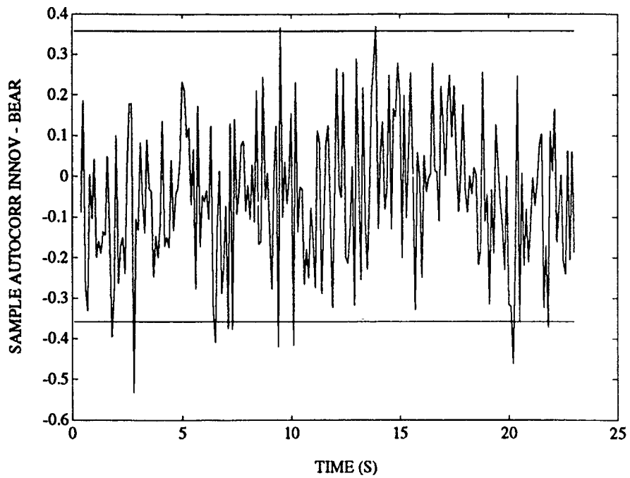
FIGURE D-39. WHITENESS TEST OF BEARING INNOVATIONS FOR 3 STATE FILTER ON S-TURN TARGET
