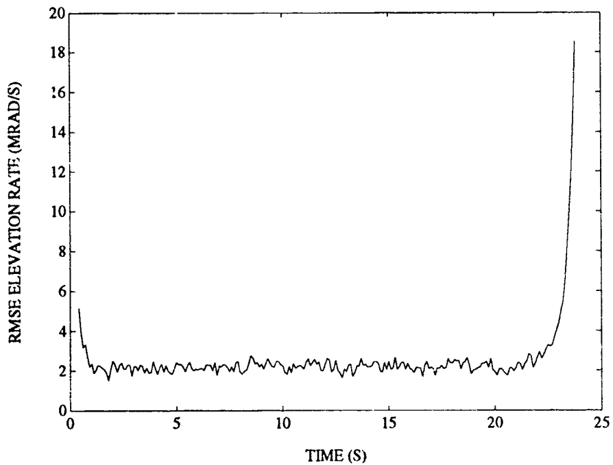
FIGURE C-50. RMS ELEVATION RATE ERROR FOR 2 STATE FILTER ON JINKING TARGET
