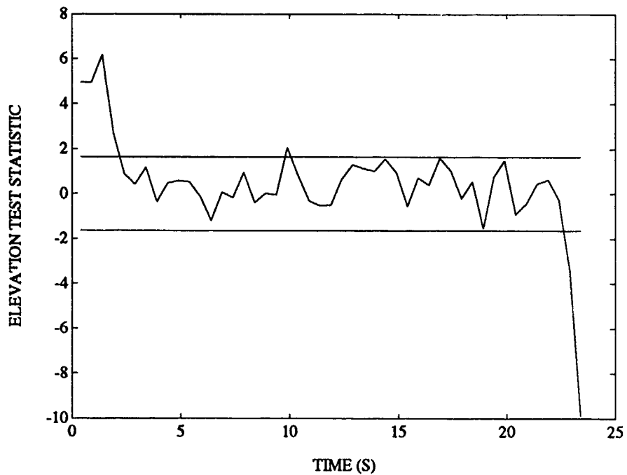
FIGURE E-15. COMPARISON OF ELEVATION ESTIMATES FROM 2 AND STATE FILTERS ON JINKING TARGET
