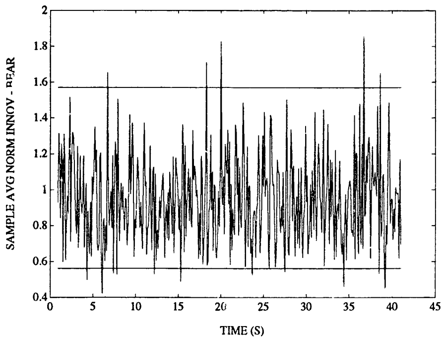
FIGURE D-23. CHI-SQUARE TEST OF BEARING INNOVATIONS FOR 3 STATE FILTER ON CROSSING TARGET
