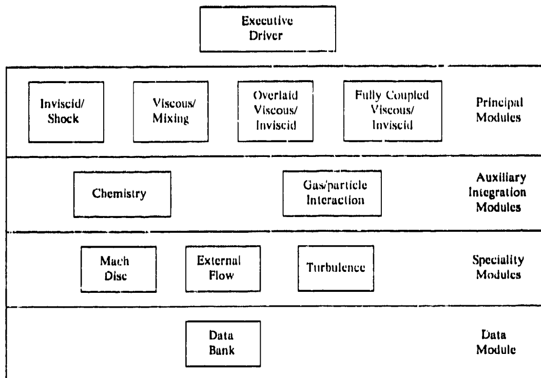
Block Schematic Modular Structure of JANNAP SPF
