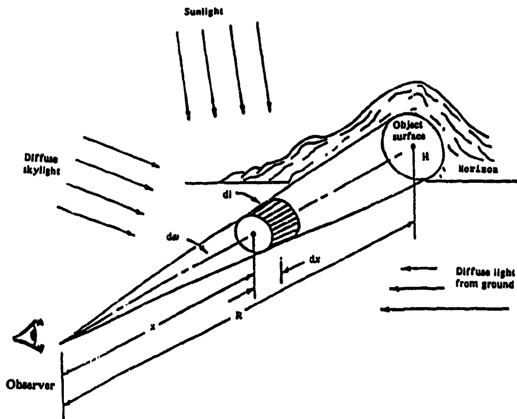
Fig. 3-8 Source of Air Light Between the Observer and an Object, and Apparent Luminance of an Object due to the Airlight [8]
