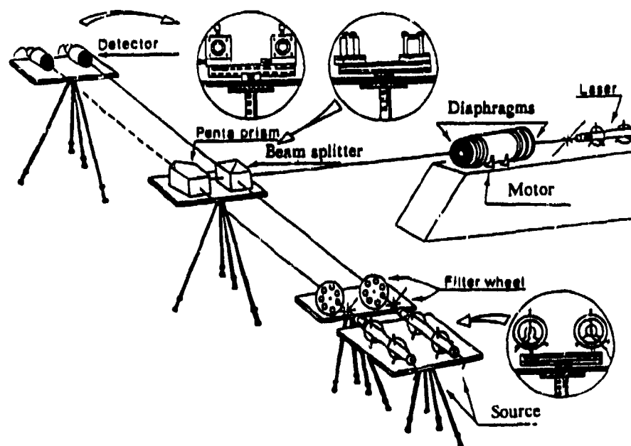
Fig. 3-9 Transmissometer at 0.6 \mu\text{m}
