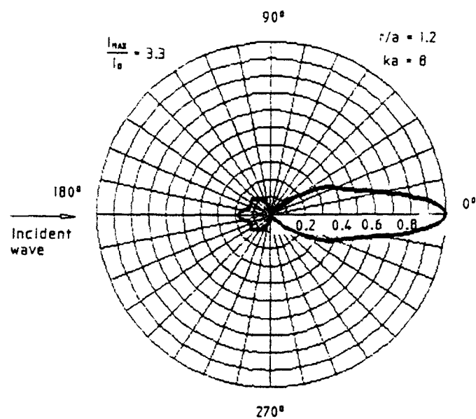
Figure 5(d): Scattered Intensity I/I_{\max} around a Rigid Sphere.
