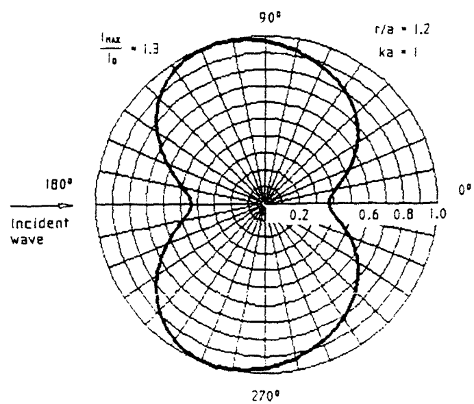
Figure 7(a): Resultant Intensity I/I_{\max} around a Rigid Sphere.
