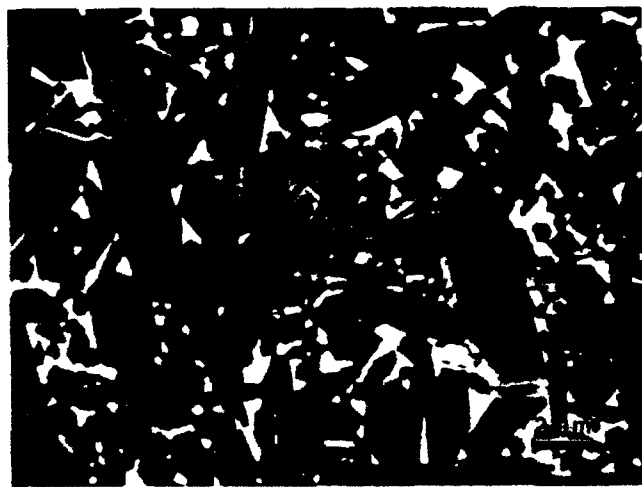
Fig. 2. SEM micrograph of cracks interacting with elongated grains in a high-toughness silicon nitride. Fracture toughness of this material is ~9 MPa·m 1/2 at a crack size of ~800 \mu m. (Courtesy C. W. Li.)
