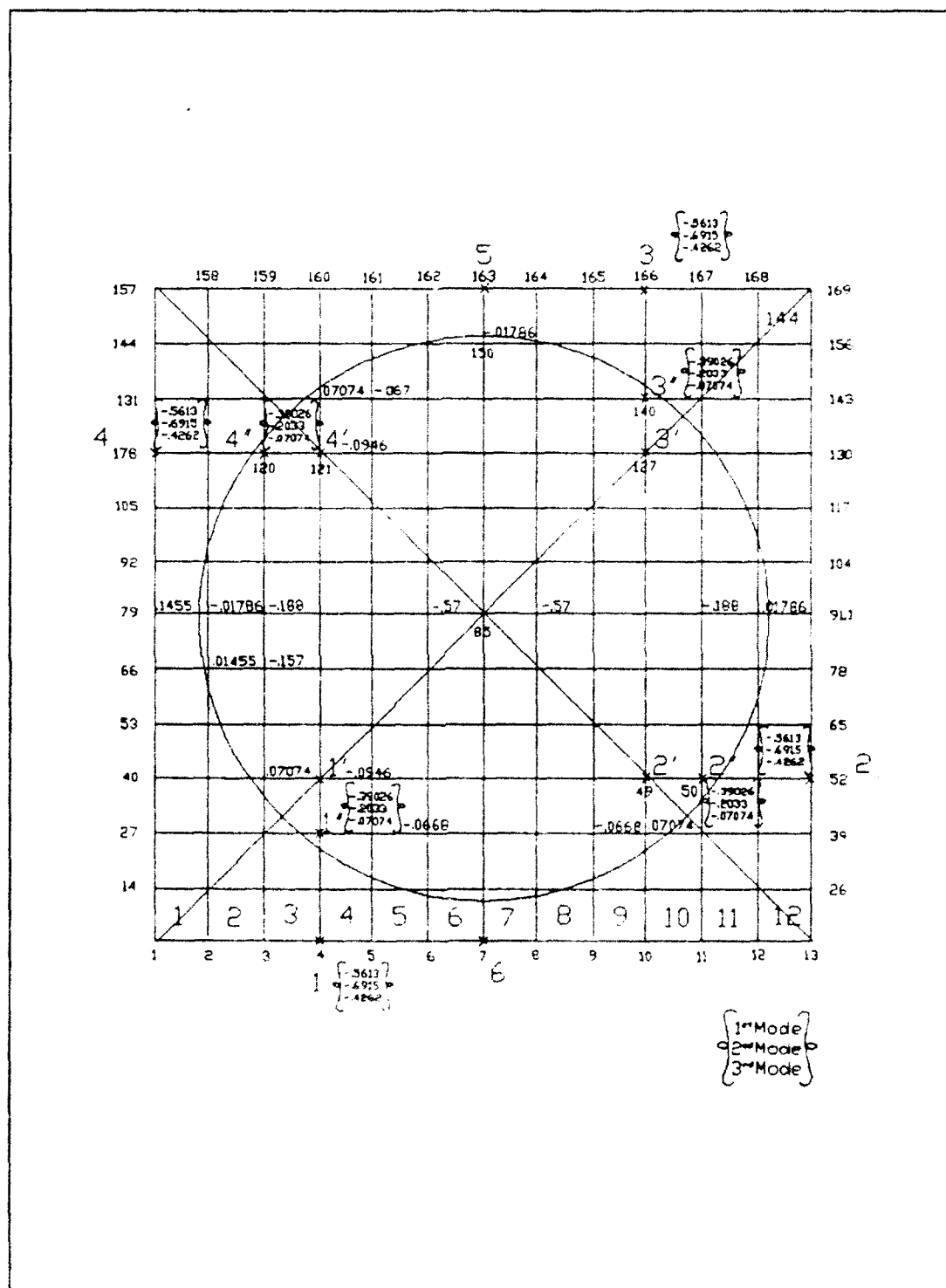
Figure 6. 144 'BPR' Finite Element Grid Pattern with Nodal Deflections for Three Different Sets of Actuator Positions
