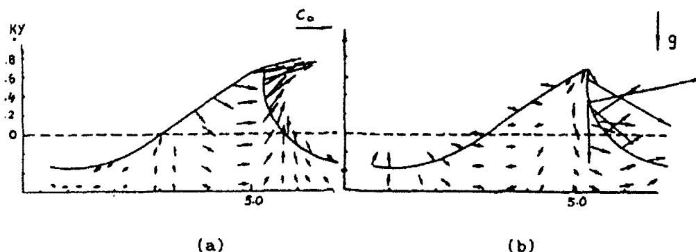
Fig.1 velocity and acceleration distributions in plunging breakers for ak = 0.44 , d=L/2 , t=0.46 (a) velocity (b) acceleration
