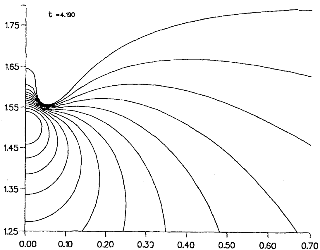
Figure 4 As for figure 3(a),(b). Pressure distribution at t = 4.19(h/g)^{1/2} the instant of maximum pressure. The contour interval is 2\rho gh . The irregularities are related to limitations in the contouring process
