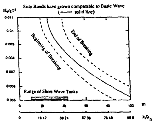
Figure 3. Regions of Breaking vs. Tank Length from Long Tank Experiments of Su & Green (1984)
