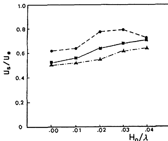
Fig.4. Dimensionless surface drift speed versus the steepness of the swell propagating against the wind. ●, U_r=3 m/s; ■, U_r=5 m/s; ▲, U_r=7 m/s.
