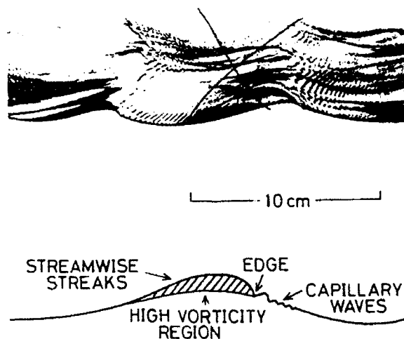
Figure 1. (from Ebuchi, Kawamura and Toba, 1987). A close-up photograph of wind-waves of length 9 cm taken with wind-speed 6 m/s at fetch 6 m. Below is a schematic picture showing the high vorticity region at the gravity wave crests.
