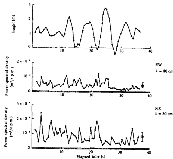
Fig. 5. Time series of power spectral density of wavenumber components during an interval embracing a whitecapping event, uncorrected for noise. Wavelength = 0.80 m. Experiment 2. Water height is with respect to an arbitrary origin. Noise levels are shown for each wavenumber component as a shaded band. 95% confidence limits about the mean level are shown at the right.
