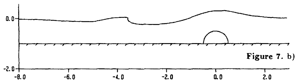
Figure 5. Flow evolution for an initial well, y = 0.20 \operatorname{sech} x , until time 80. Figure 6. Detail of the breaking profile; the flow is started with an initial well, y = 0.35 \operatorname{sech} x , at time 6.75. The breaking crest is 0.21 high, the maximum slope is 156^\circ . Figure 7. Downstream breakers for semi-circular cylinders. a) r = 0.3 and F = 1.0 time 55.8, the breaking crest is 0.399 high at x = -13.0 , the maximum slope is 123.78^\circ . b) r = 0.5 and F = 1.6 at time 2.50, the breaking crest is 0.070 high at x = -3.7 , the maximum slope is 145.41^\circ .
