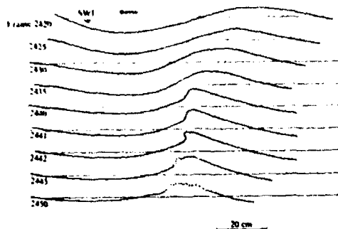
Figure 1. Evolution of a Wave Leading to Breaking (with frame frequency 24 f/s) from Tank Experiments of Bonmarin (1989)
