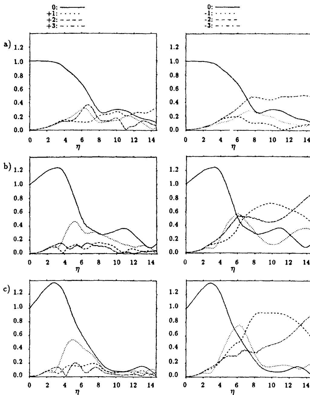
Figure 3: Evolution of wavetrain for different wind velocities. The two columns show spectral development with upper sidebands (left column) and lower sidebands (right column). In a) u_*/c = 0 , b) u_*/c = 0.33 and c) u_*/c = 0.40
