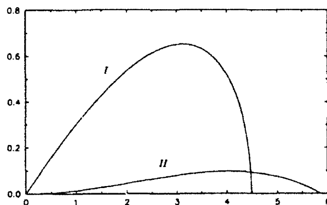
Figure 2: Growth rate of the M.I. as a function of perturbation wavenumber. I: for initial wave steepness 0.23 and u_* = 0 . II: for wave steepness kA_c(1 + \beta\tau)^{1/r} (slightly supercritical).
