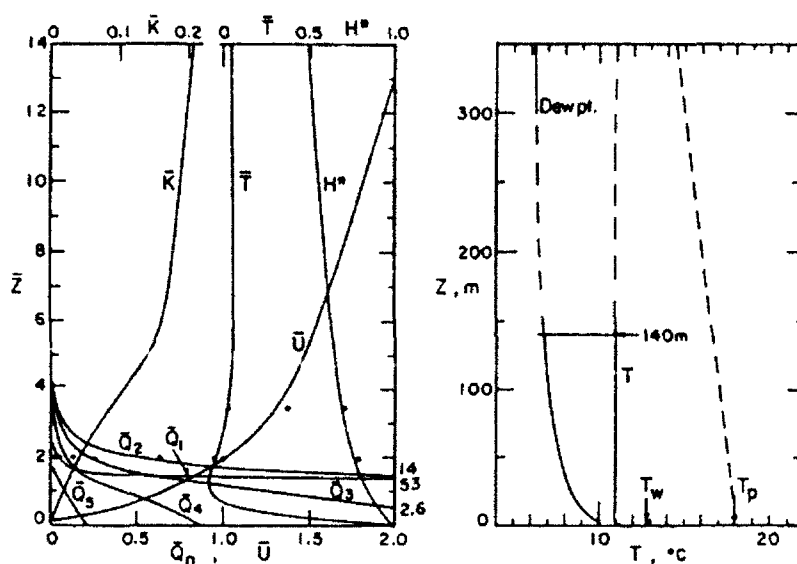
Fig. 2. Sounding August 20th, 15:45; U_{10}=15.6 m/s, 190^\circ ; z_0=140 m; T_0=11.0^\circ\text{C} ; H_0^*=0.40 ; T_w=12.8^\circ\text{C} ; q_w=4.7 \times 10^{-4} kg/m 2 s; h_l=280 cal/m 2 s; Bowen ratio = -0.2 at \bar{z}=6 ; storm.
