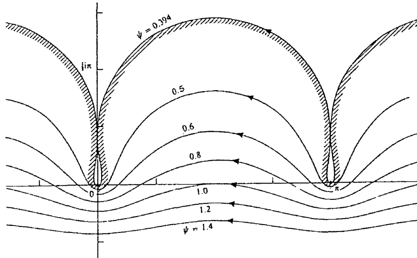
Figure 5. (from Longuet-Higgins 1988). Streamlines and free surfaces in Crapper's solution for an irrotational, pure capillary wave, viewed in a frame of reference moving to the right with the phase-speed c . Units are dimensionless, with c = 1, k = 2 .
