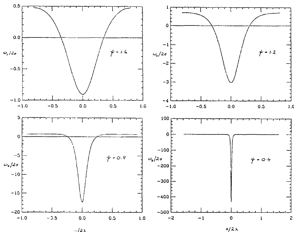
Figure 6. The vorticity \omega_s generated at the surface of a pure capillary wave (Figure 5). (a) \psi_0 = 1.6 , (b) \psi_0 = 1.2 , (c) \psi_0 = 0.8 , (d) \psi_0 = 0.4 .
