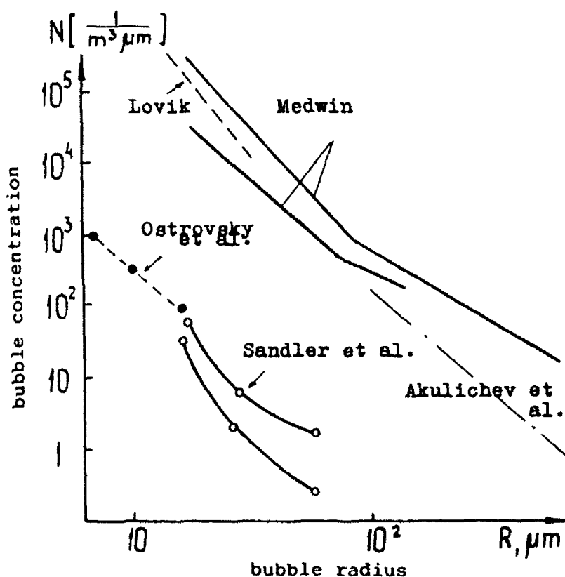
Fig. 1. Ocean measurements of bubble concentration.
