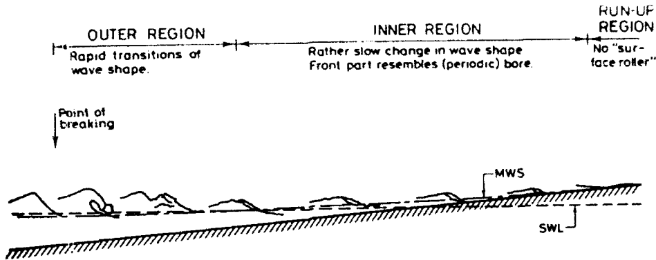
Figure 1: Wave characteristics in the surf zone (from Svendsen et al., 1978).
