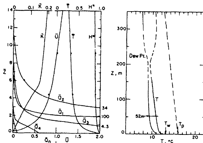
Fig. 1. Sounding August 7th, 18:18: U_{10}=6.3 m/s, 350^\circ ; z_0=52 m; T_0=10.8^\circ\text{C} ; H_0^*=0.78 ; T_w=13.2^\circ\text{C} ; q_w=5.4 \times 10^{-5} kg/m 2 s; h_l=32 cal/m 2 s; Bowen ratio=0.23 at \bar{z}=6 .
