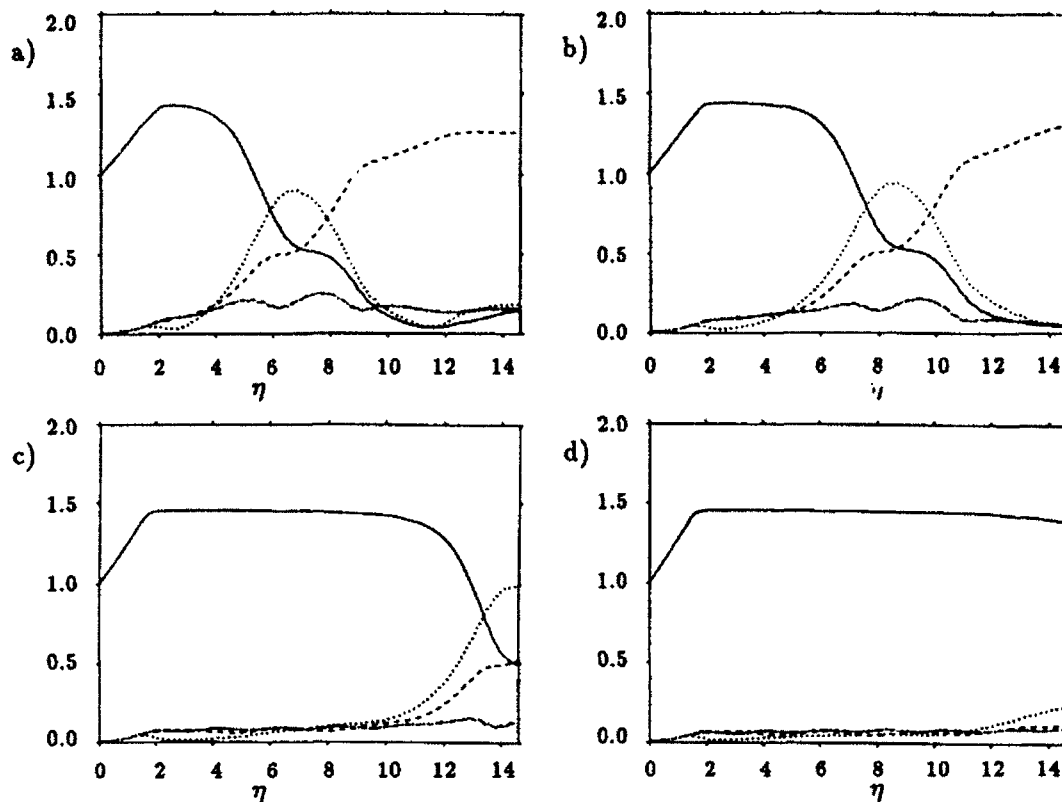
Figure 4: Spectral development of carrier and lower sidebands for different u_*/c a) 0.46 b) 0.48 c) 0.50 d) 0.52
