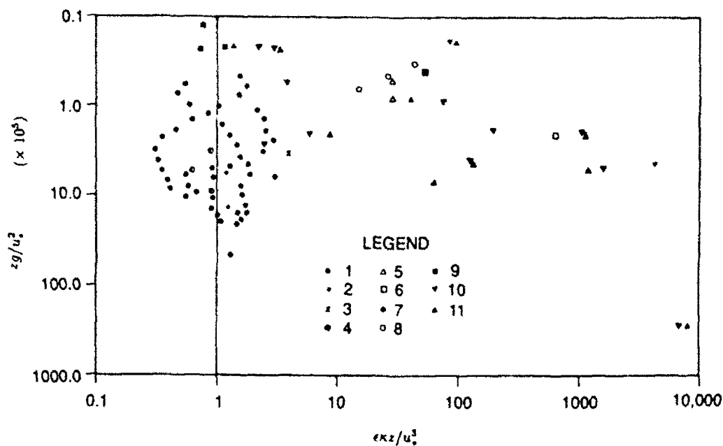
Figure 2: Dissipation in 'wall layer' coordinates, with the 'law of the wall' as a vertical line (—). Symbols: \circ \triangle \square from [1], \times [2], \bullet [3], \blacksquare \blacktriangledown \blacktriangle this experiment. + \blacklozenge and \circ as given in [3].
