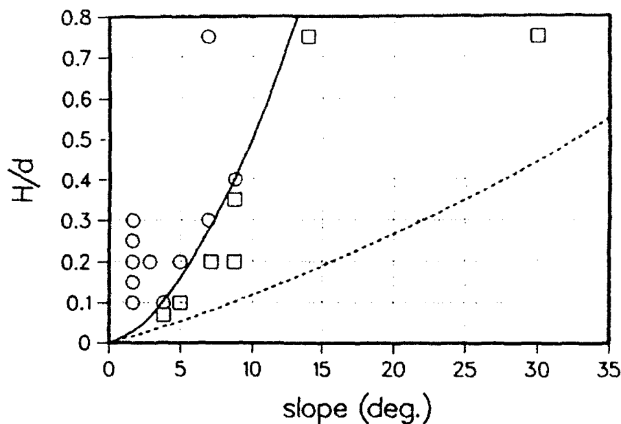
Figure 4: Breaking limit for solitary waves on slopes. ○ breaking waves, □ non-breaking, - - - (3), — (4)
