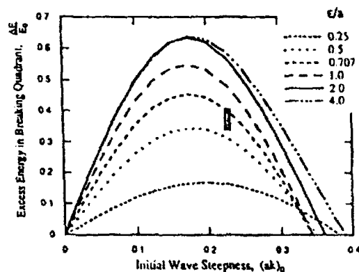
Figure 6. Excess Energy in Breaking Quadrant [□ data of Melville(1982), (ak)_0=0.23 , (\epsilon/a)_m=1/\sqrt{2} ]
