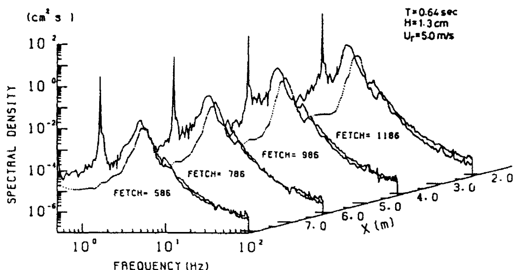
Fig.2. Comparison of the wave spectra of the co-existent system (solid line) and those of pure wind waves (dotted line). swell, T=0.64\text{sec} , H=1.3\text{cm} ; wind speed, U_x=5\text{m/s} .
