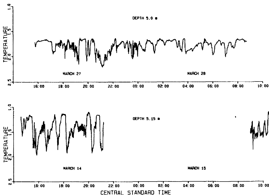
Fig. 2. Time history of temperature in the Waskesiu Narrows March 14-15 and March 27-28, 1991. The amplitude of the internal wave activity varied from day to night and from week to week with changes in the incident radiation.
