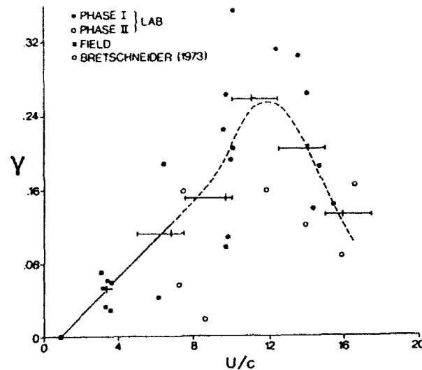
Fig. 2. The fraction of wind momentum retained by waves \gamma versus the inverse wave age U/c . For the laboratory data the larger crosses indicate the averages of the data assembled in groups of width 2.5 in U/c . The vertical bar indicates the average value of U/c in the group. The cross representing the field data has been placed at the value of \gamma corresponding to neutral atmospheric stability. The point of full development ( U/c = 0.83 , \gamma = 0 ) according to Bretschneider (1973) provides another estimate of \gamma . The straight line (solid) at lower values of U/c provides convenient access to \gamma for wave prediction purposes. The extension of the line to higher values of U/c (dashed) serves only to illustrate the trend in \gamma .
