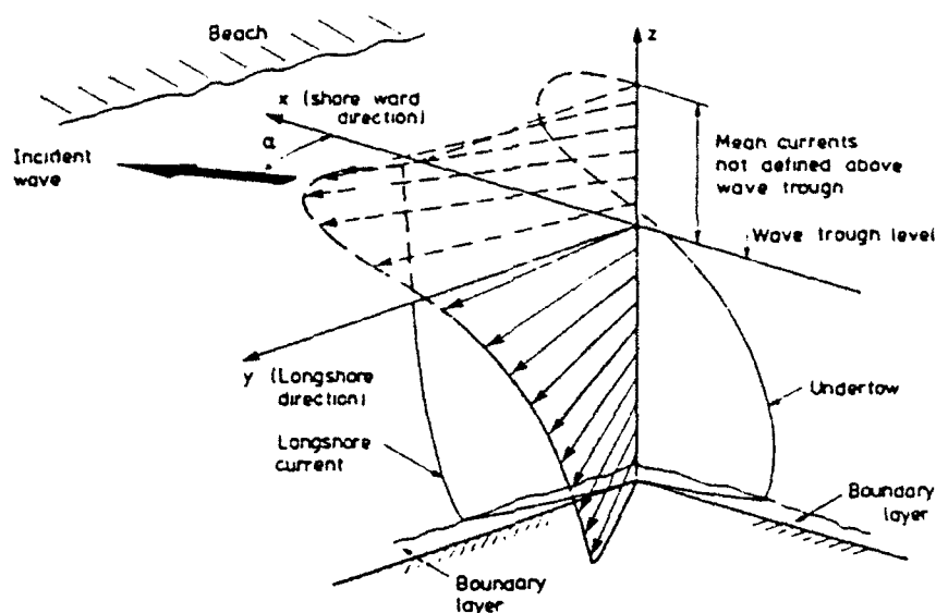
Figure 2: The three dimensional structure of surf zone current profiles (from Svendsen & Lorenz, 1989).
