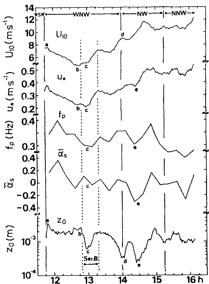
Fig.2. The 4-hr. time series of U_{10} , u_* , the wind-wave peak frequency f_p , the degree of under-saturation \alpha_s defined by Eq.(1), and the roughness length z_0 . The data of U_{10} , u_* and z_0 are from the 15-min. moving average wind speeds.
