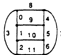
Figure 3. A 3-cube C_3
