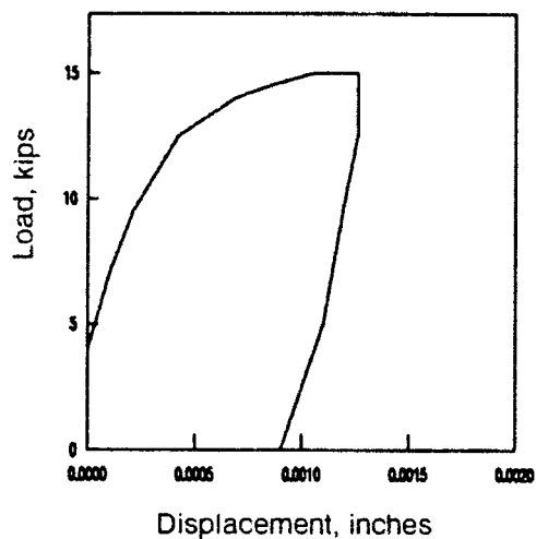
Figure 2.9 Typical Shear Force-Deflection Curve for Shove Test
