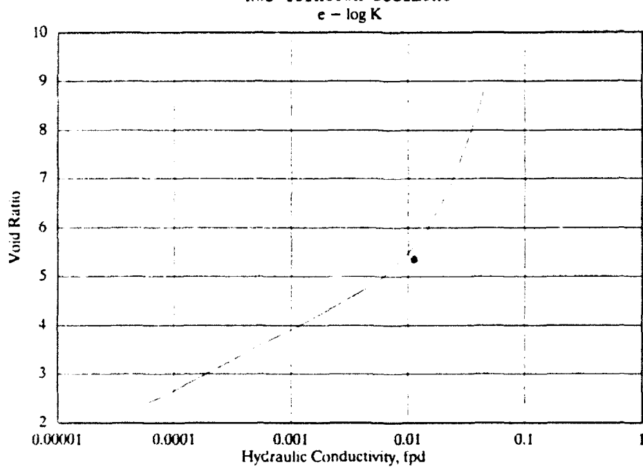
Figure 44. Void ratio-permeability relationship for NWS Yorktown sediment
