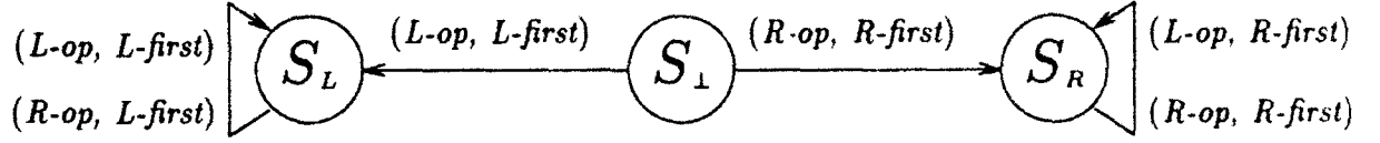
Figure 4: Object type T_{\text{sticky}}
